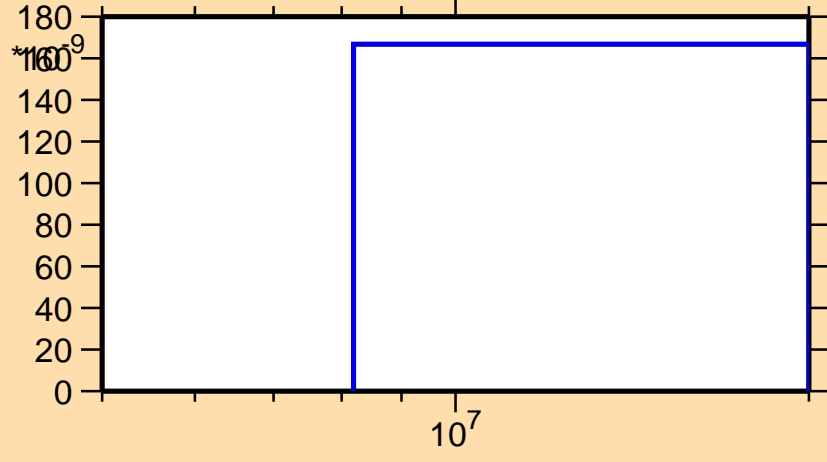
\sigma vs. E for ^{97}\text{Ru}(n,nd)
