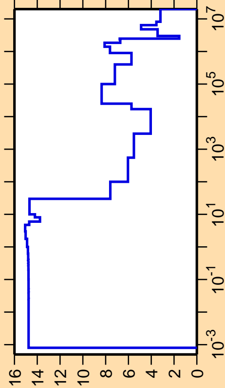
\Delta\sigma/\sigma vs. E for ^{97}\text{Ru}(n,\text{el.})
