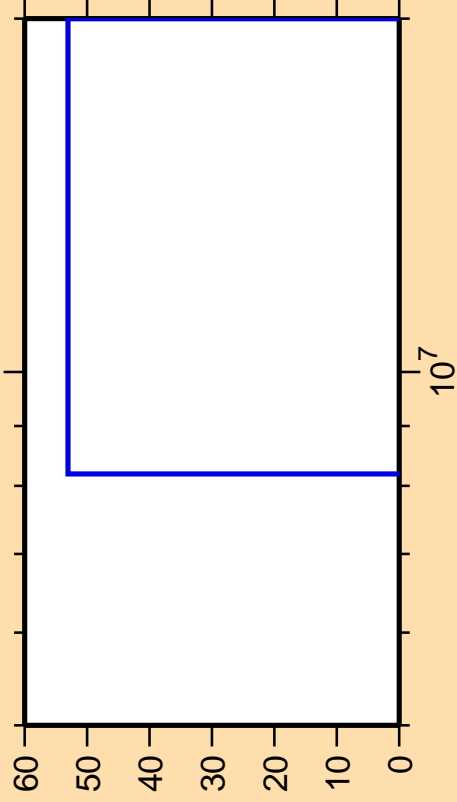
\Delta\sigma/\sigma vs. E for ^{97}\text{Ru}(n,nd)
