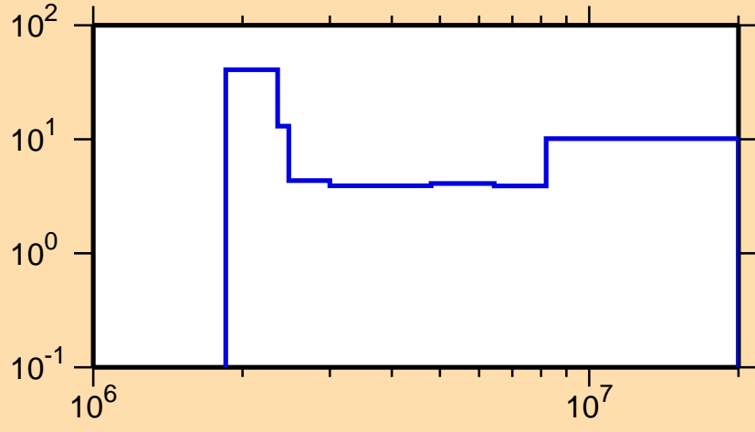
\Delta\sigma/\sigma vs. E for ^{97}\text{Ru}(n,n\text{cont.})
