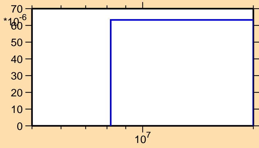
\sigma vs. E for ^{97}\text{Ru}(n,t)
