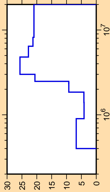
\Delta\sigma/\sigma vs. E for ^{97}\text{Ru}(n,n_3)
