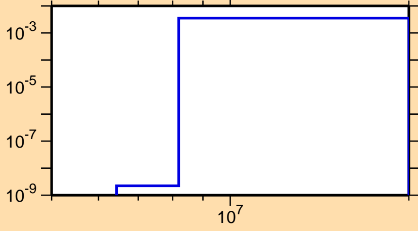
\sigma vs. E for ^{97}\text{Ru}(n,d)
