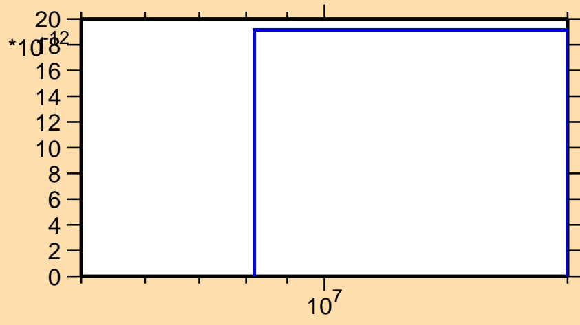
\sigma vs. E for ^{97}\text{Ru} (mt 45)
