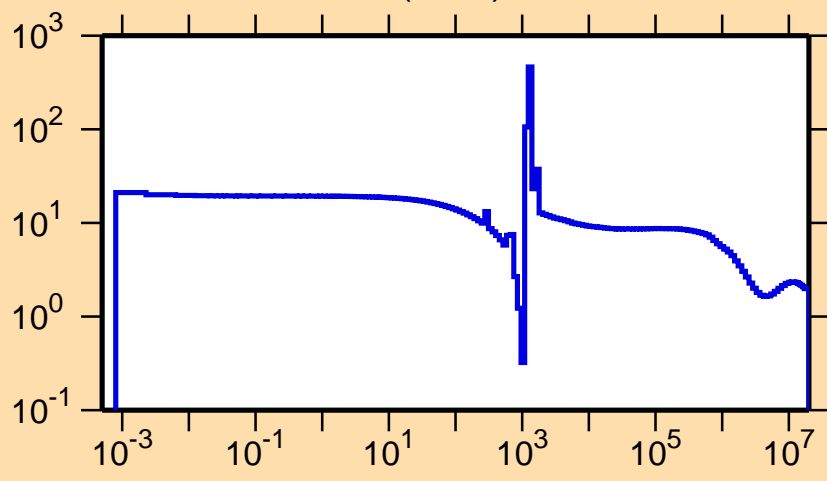
\sigma vs. E for ^{98}\text{Ru}(n,\text{el.})
