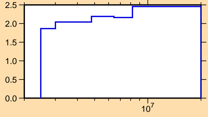
\Delta\sigma/\sigma vs. E for ^{98}\text{Ru}(n,n\text{onel.})
