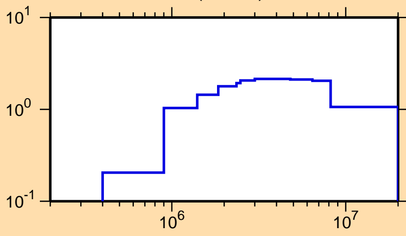
\sigma vs. E for ^{98}\text{Ru}(n,\text{inel.})
