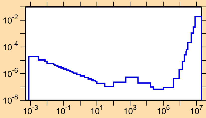
\sigma vs. E for ^{98}\text{Ru}(n,\alpha)
