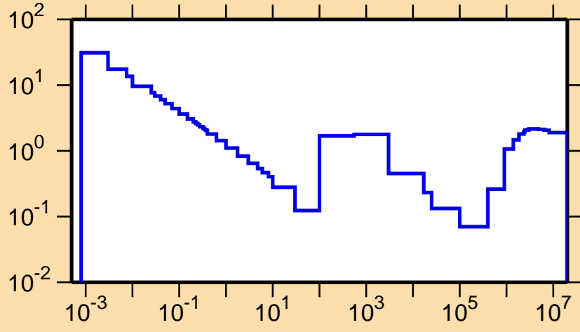
\sigma vs. E for ^{98}\text{Ru}(n,\text{nonel.})
