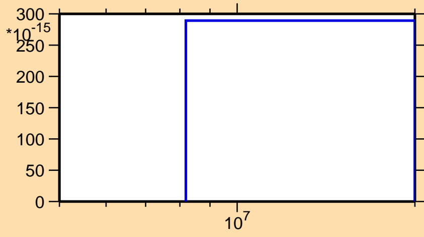
\sigma vs. E for ^{99}\text{Ru}(n,nt)
