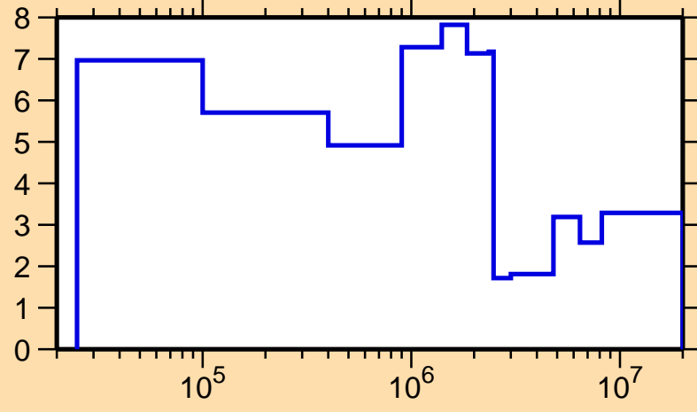
\Delta\sigma/\sigma vs. E for ^{99}\text{Ru}(n,\text{el.})
