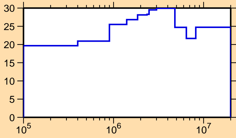
\Delta\sigma/\sigma vs. E for ^{99}\text{Ru}(n,\gamma)
