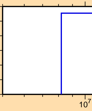
\sigma vs. E for ^{99}\text{Ru} (mt 34)
