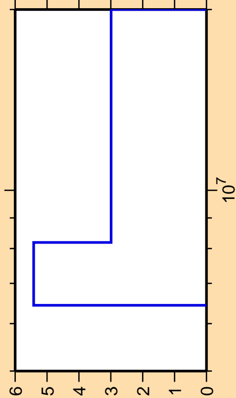
\Delta\sigma/\sigma vs. E for ^{99}\text{Ru}(n,2n)
