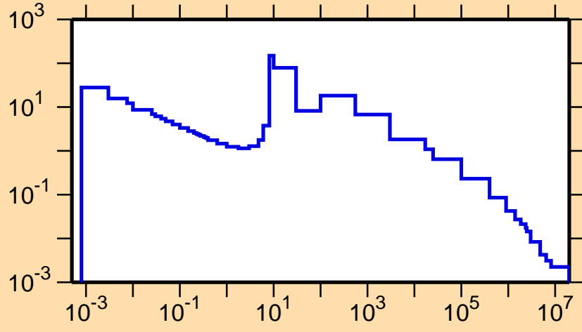
\sigma vs. E for ^{99}\text{Ru}(n,\gamma)
