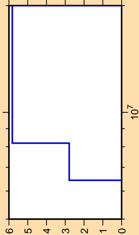
\Delta\sigma/\sigma vs. E for ^{99}\text{Ru}(n,n\text{cont.})
