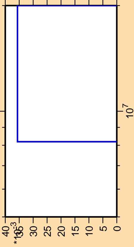
\Delta\sigma/\sigma vs. E for ^{99}\text{Ru}(n,\text{pd})
