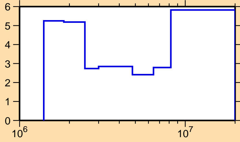
\Delta\sigma/\sigma vs. E for ^{99}\text{Ru}(n,ncont.)
