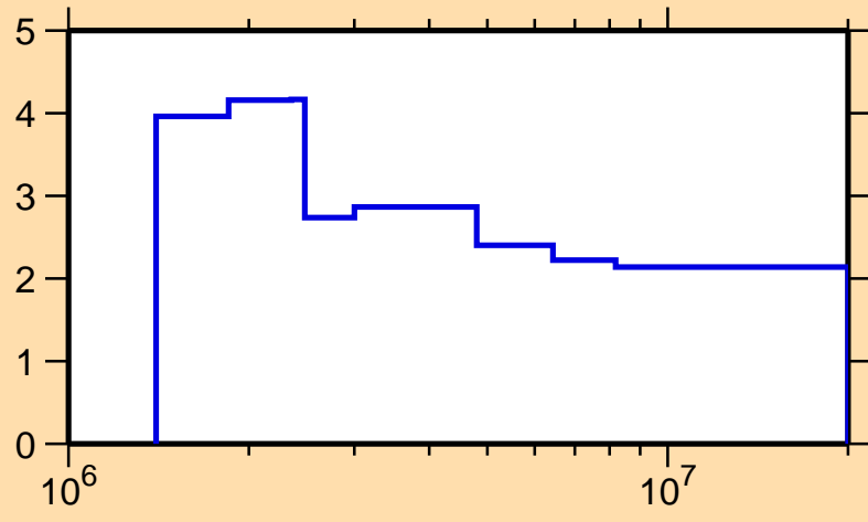
\Delta\sigma/\sigma vs. E for ^{99}\text{Ru}(n,n\text{onel.})
