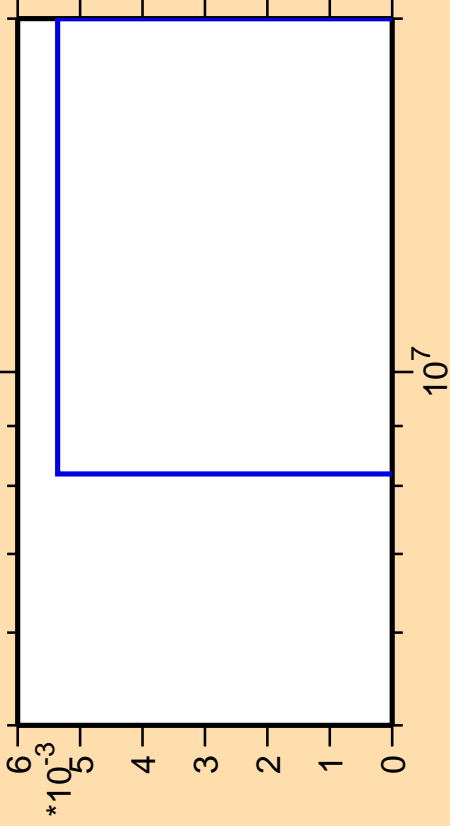
\Delta\sigma/\sigma vs. E for ^{99}\text{Ru}(\text{mt117})
