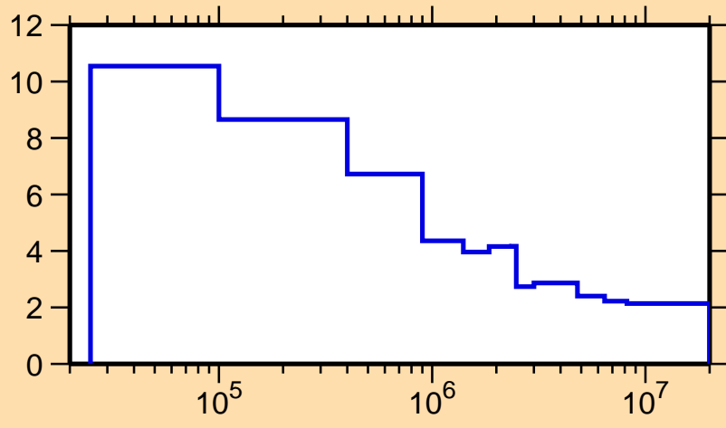
\Delta\sigma/\sigma vs. E for ^{99}\text{Ru}(n,\text{nonel.})
