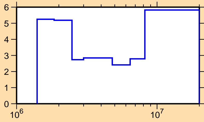
\Delta\sigma/\sigma vs. E for ^{99}\text{Ru}(n,n\text{cont.})
