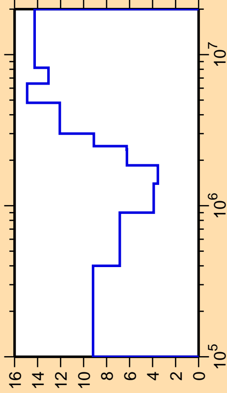
\Delta\sigma/\sigma vs. E for ^{99}\text{Ru}(n,n_3)
