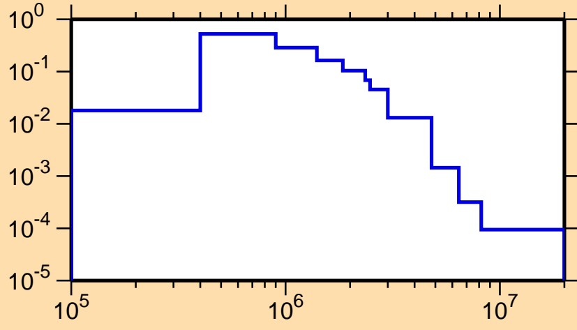
\sigma vs. E for ^{99}\text{Ru}(n,n_3)
