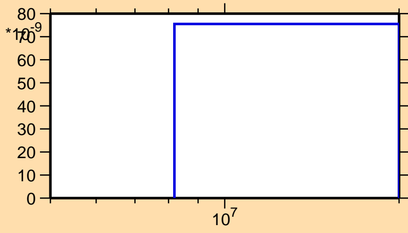
\sigma vs. E for ^{99}\text{Ru}(n,nd)
