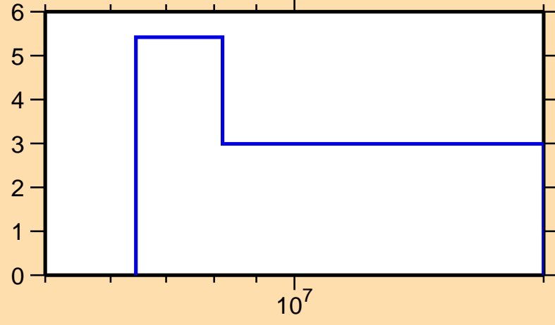
\Delta\sigma/\sigma vs. E for ^{99}\text{Ru}(n,2n)
