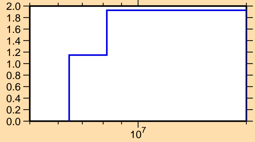
\Delta\sigma/\sigma vs. E for ^{99}\text{Ru}(n,\text{tot.})
