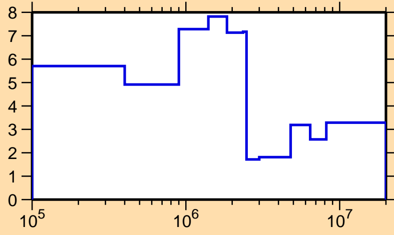
\Delta\sigma/\sigma vs. E for ^{99}\text{Ru}(n,el.)
