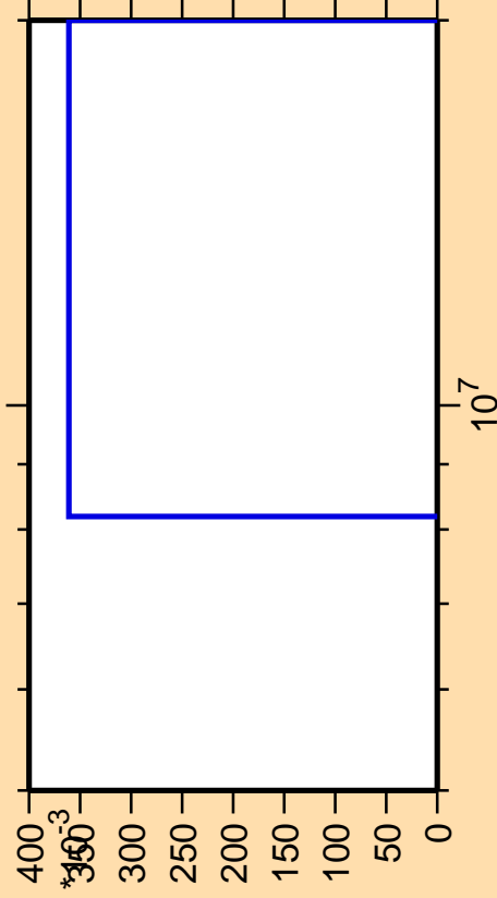
\Delta\sigma/\sigma vs. E for ^{99}\text{Ru}(n,nt)
