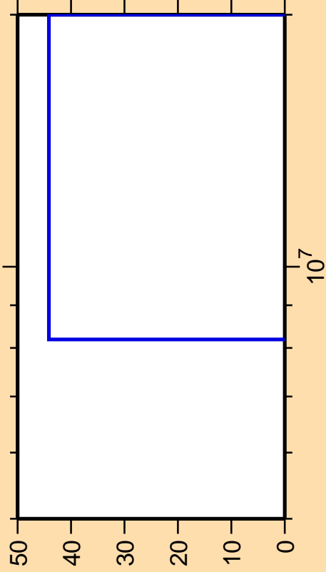
\Delta\sigma/\sigma vs. E for ^{99}\text{Ru}(n,nd)
