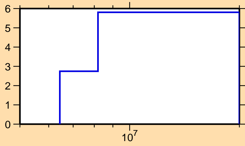
\Delta\sigma/\sigma vs. E for ^{99}\text{Ru}(n,\text{inel.})
