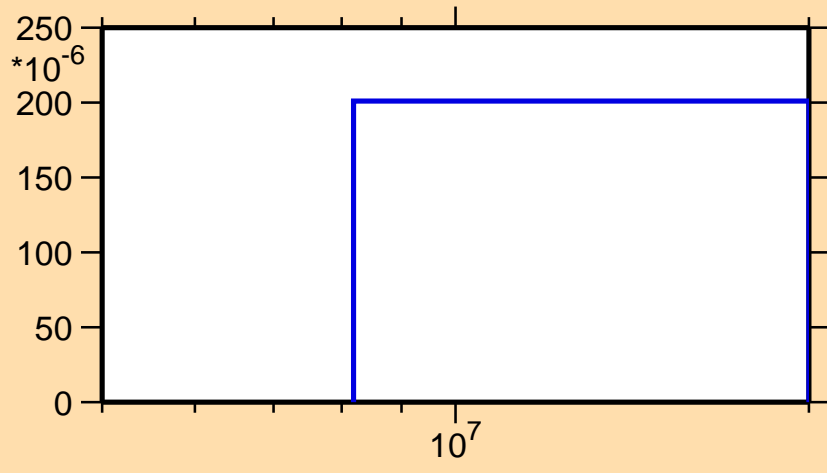
\sigma vs. E for ^{99}\text{Ru}(n,t)
