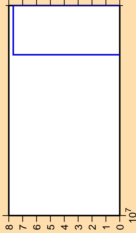
\Delta\sigma/\sigma vs. E for ^{100}\text{Ru}(n,2np)
