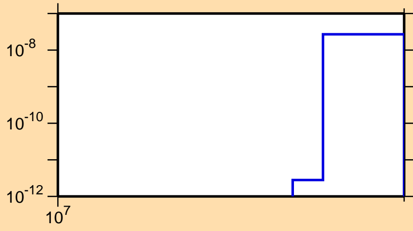
\sigma vs. E for ^{100}\text{Ru}(n,nd)
