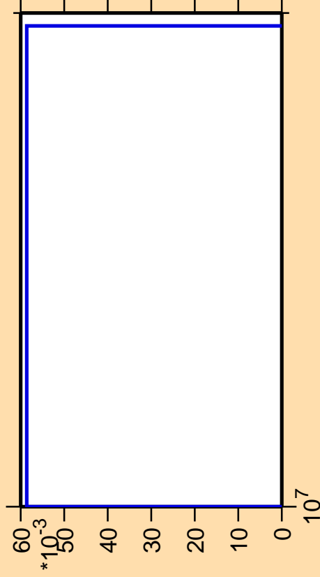
\Delta\sigma/\sigma vs. E for ^{100}\text{Ru}(n,2np)
