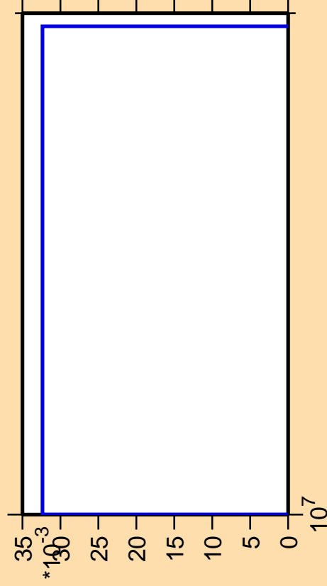
\Delta\sigma/\sigma vs. E for ^{100}\text{Ru}(n,nt)
