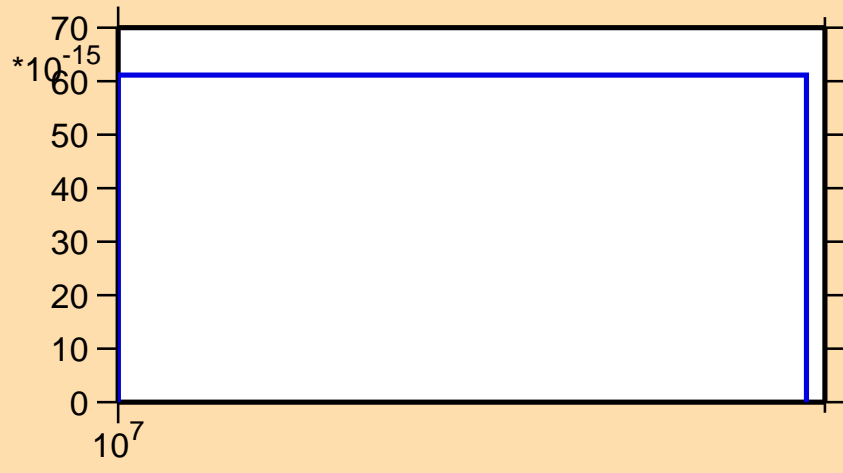
\sigma vs. E for ^{100}\text{Ru}(n,2np)
