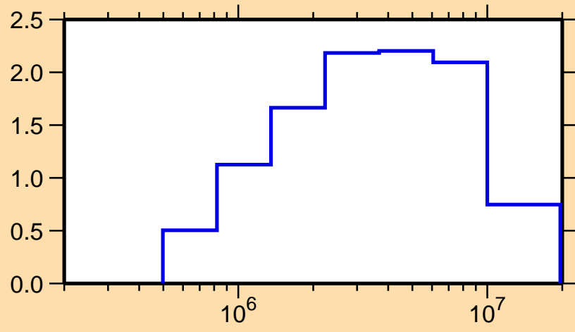
\sigma vs. E for ^{100}\text{Ru}(n,\text{inel.})
