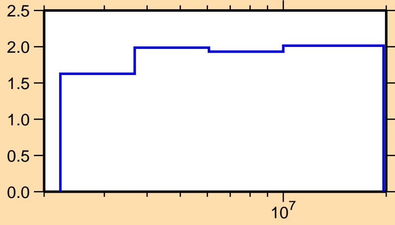
\Delta\sigma/\sigma vs. E for ^{100}\text{Ru}(n,n\text{onel.})
