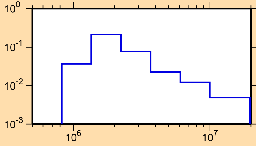
\sigma vs. E for ^{100}\text{Ru}(n,n_2)
