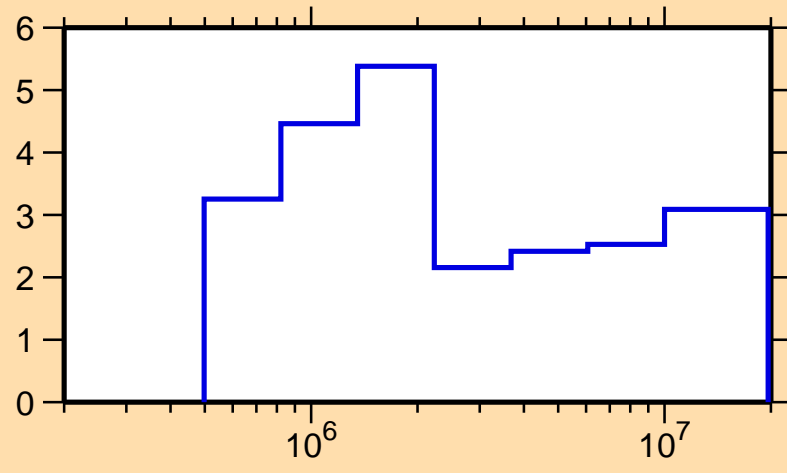
\Delta\sigma/\sigma vs. E for ^{100}\text{Ru}(n,\text{el.})
