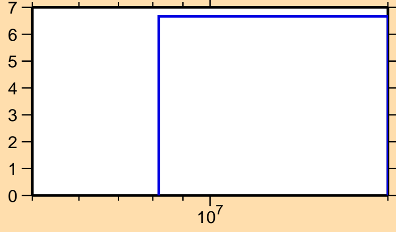
\Delta\sigma/\sigma vs. E for ^{100}\text{Ru}(n,\text{inel.})
