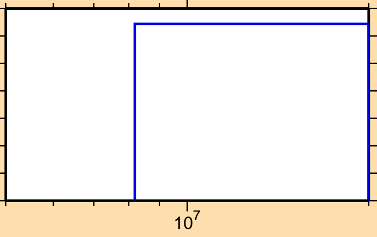
\sigma vs. E for ^{100}\text{Ru}(n,np)
