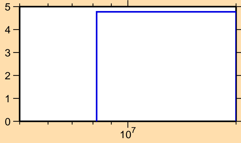
\Delta\sigma/\sigma vs. E for ^{100}\text{Ru}(n,2n)
