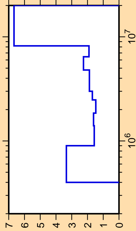
\Delta\sigma/\sigma vs. E for ^{100}\text{Ru}(n,\text{inel.})
