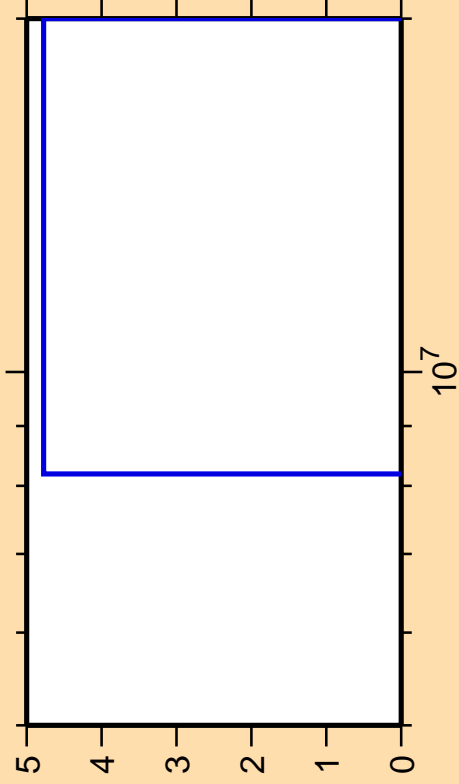
\Delta\sigma/\sigma vs. E for ^{100}\text{Ru}(n,2n)
