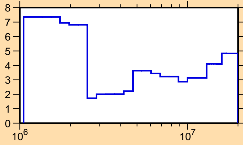
\Delta\sigma/\sigma vs. E for ^{101}\text{Ru}(n,\text{el.})
