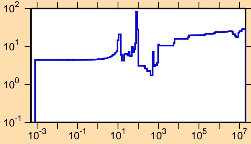
\Delta\sigma/\sigma vs. E for ^{101}\text{Ru}(n,\gamma)
