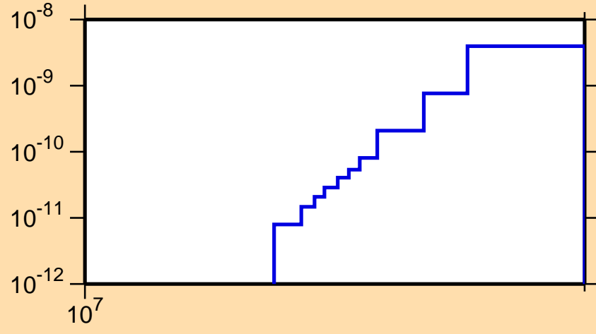
\sigma vs. E for ^{101}\text{Ru}(n,p\alpha)
