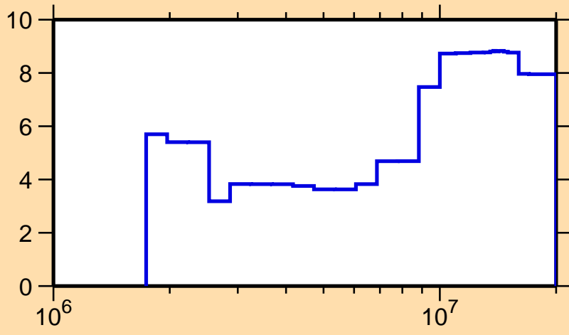
\Delta\sigma/\sigma vs. E for ^{101}\text{Ru}(n,n\text{cont.})
