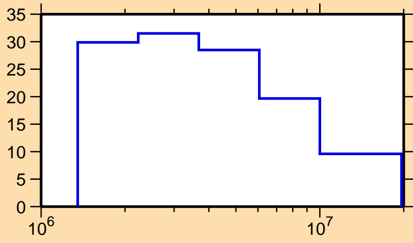
\Delta\sigma/\sigma vs. E for ^{101}\text{Ru}(n,p)
