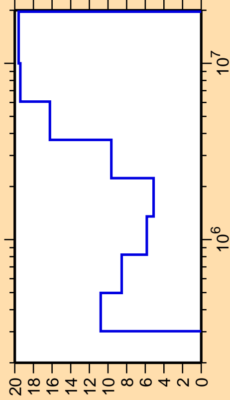
\Delta\sigma/\sigma vs. E for ^{101}\text{Ru}(n,n_2)
