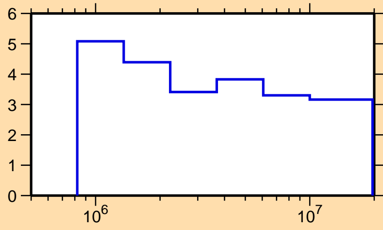
\Delta\sigma/\sigma vs. E for ^{101}\text{Ru}(n,n\text{onel.})
