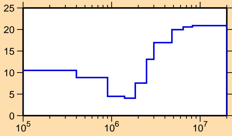
\Delta\sigma/\sigma vs. E for ^{101}\text{Ru}(n,n_1)
