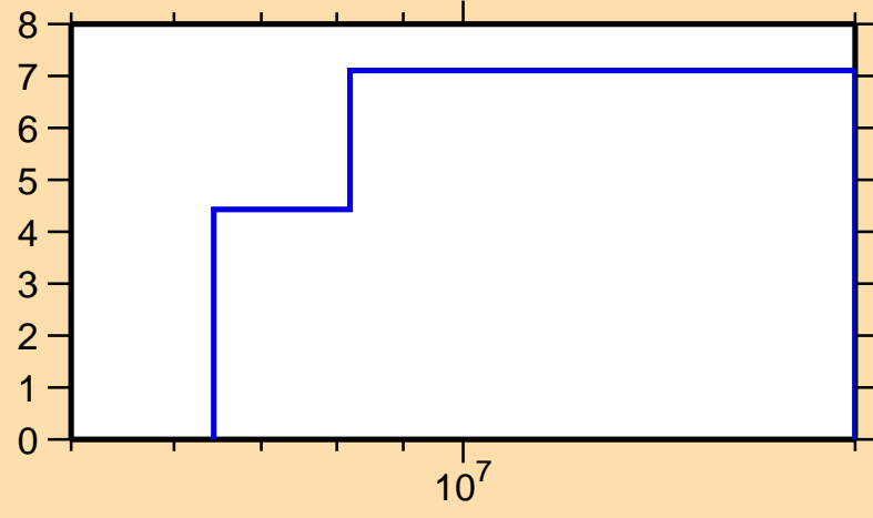
\Delta\sigma/\sigma vs. E for ^{101}\text{Ru}(n,\text{inel.})
