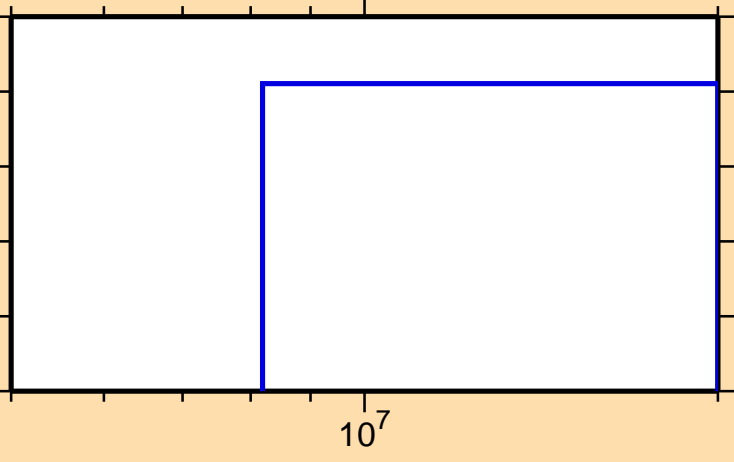
\sigma vs. E for ^{101}\text{Ru}(n,2np)
