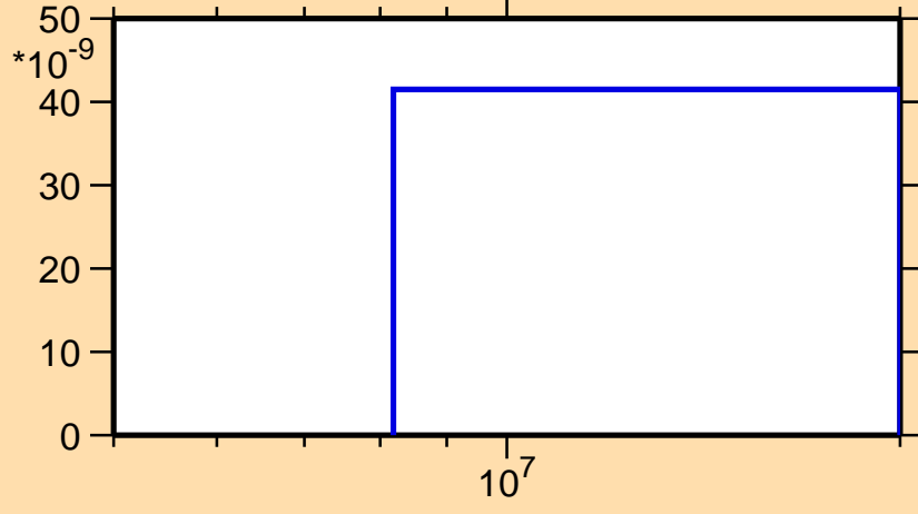
\sigma vs. E for ^{101}\text{Ru}(n,nd)
