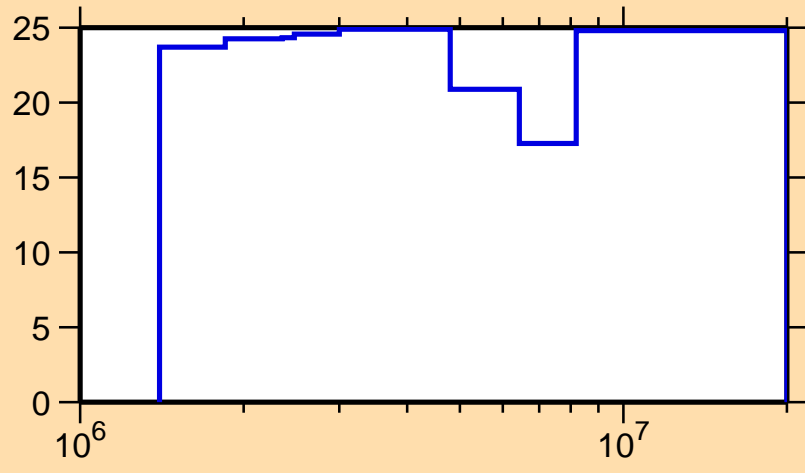
\Delta\sigma/\sigma vs. E for ^{101}\text{Ru}(n,\gamma)
