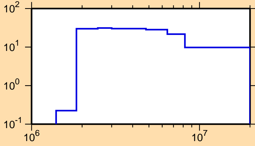
\Delta\sigma/\sigma vs. E for ^{101}\text{Ru}(n,p)
