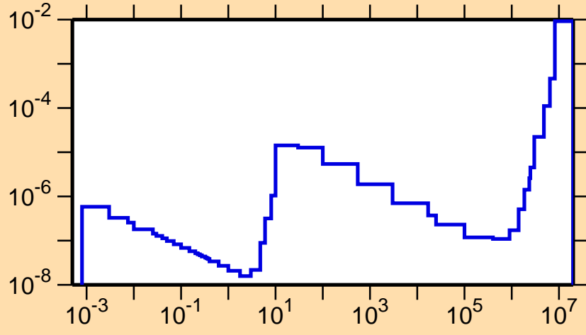
\sigma vs. E for ^{101}\text{Ru}(n,\alpha)
