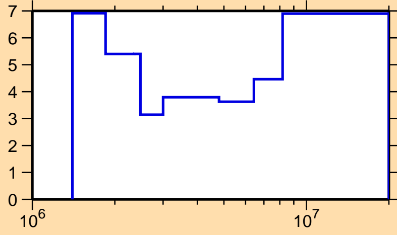
\Delta\sigma/\sigma vs. E for ^{101}\text{Ru}(n,n\text{cont.})
