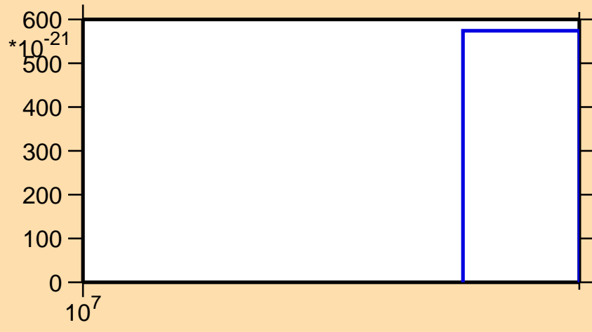
\sigma vs. E for ^{102}\text{Ru} (mt 34)
