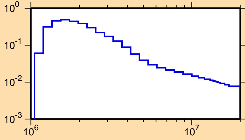
\sigma vs. E for ^{102}\text{Ru}(n,n_3)
