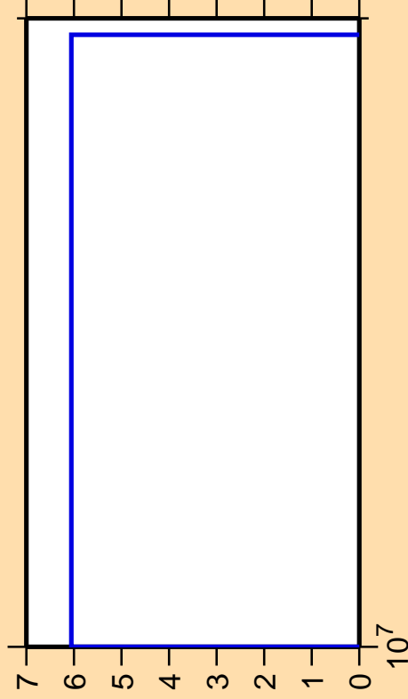
\Delta\sigma/\sigma vs. E for ^{102}\text{Ru}(n,2n\alpha)
