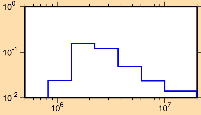
\sigma vs. E for ^{102}\text{Ru}(n,n_4)
