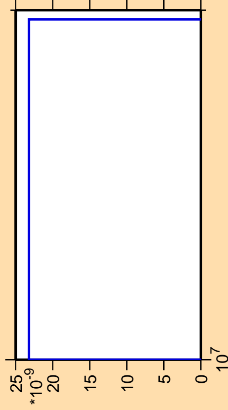
\Delta\sigma/\sigma vs. E for ^{102}\text{Ru} (mt 34)
