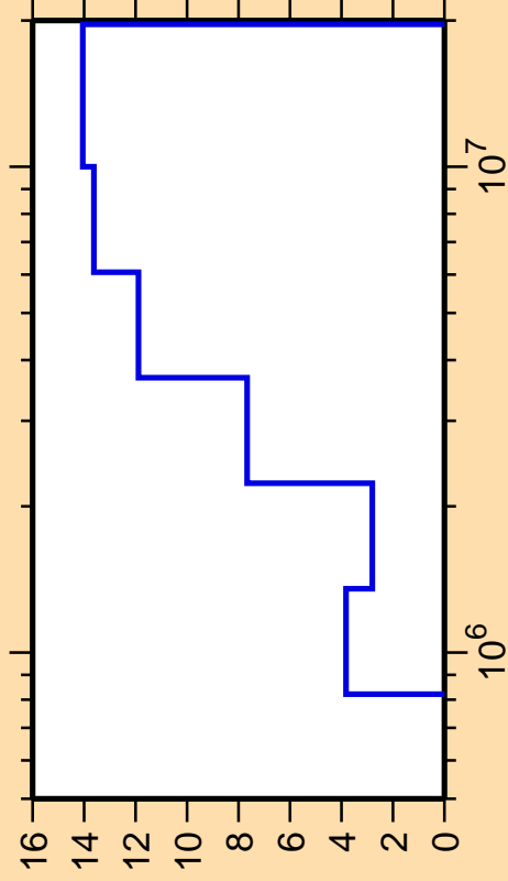
\Delta\sigma/\sigma vs. E for ^{102}\text{Ru}(n,n_4)
