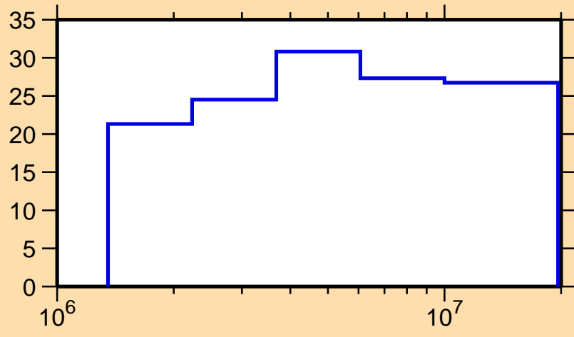
\Delta\sigma/\sigma vs. E for ^{102}\text{Ru}(n,\gamma)
