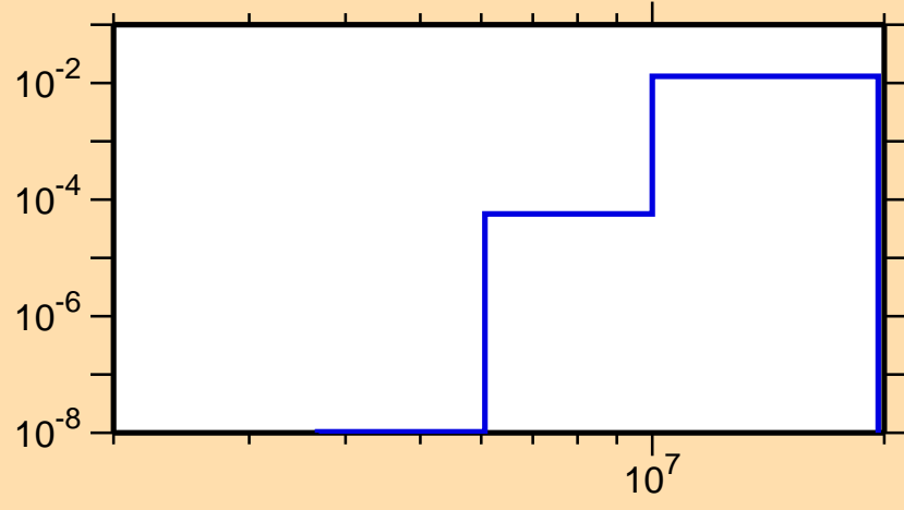
\sigma vs. E for ^{102}\text{Ru}(n,p)
