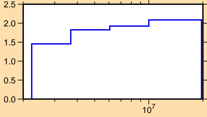
\Delta\sigma/\sigma vs. E for ^{102}\text{Ru}(n,n\text{onel.})
