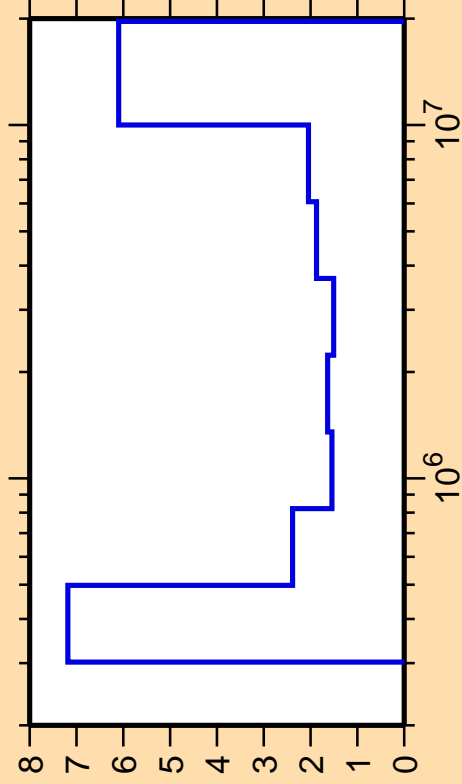
\Delta\sigma/\sigma vs. E for ^{102}\text{Ru}(n,\text{inel.})
