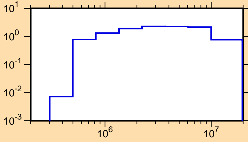
\sigma vs. E for ^{102}\text{Ru}(n,\text{inel.})
