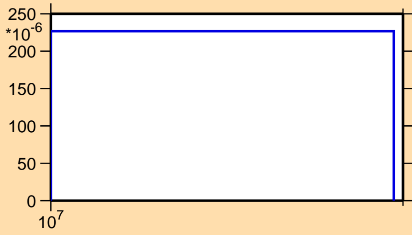
\sigma vs. E for ^{102}\text{Ru}(n,3n)
