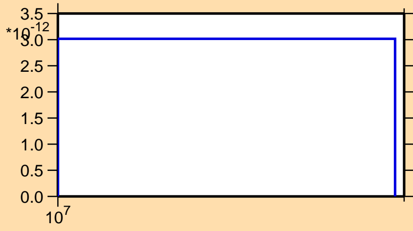
\sigma vs. E for ^{102}\text{Ru}(n,\text{He3})
