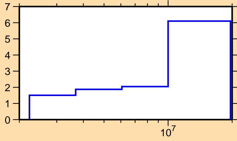
\Delta\sigma/\sigma vs. E for ^{102}\text{Ru}(n,\text{inel.})
