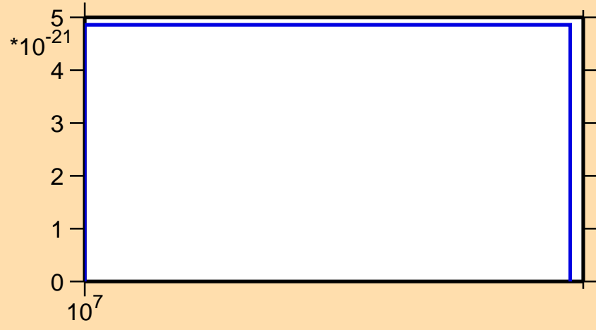
\sigma vs. E for ^{102}\text{Ru} (mt 34)
