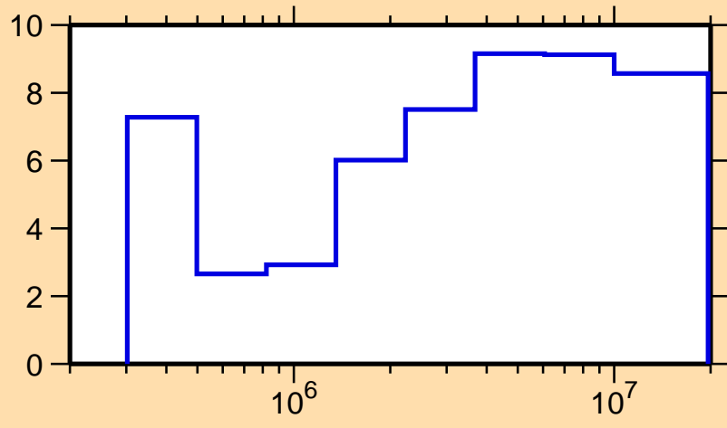
\Delta\sigma/\sigma vs. E for ^{102}\text{Ru}(n,n_1)
