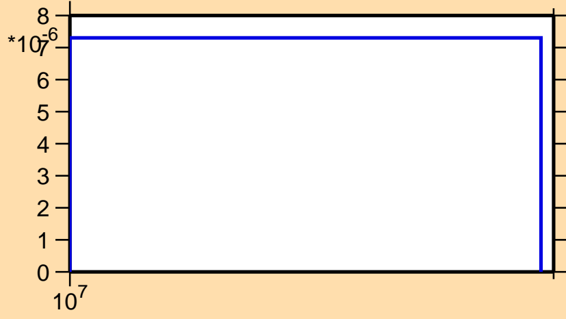
\sigma vs. E for ^{102}\text{Ru}(n,t)
