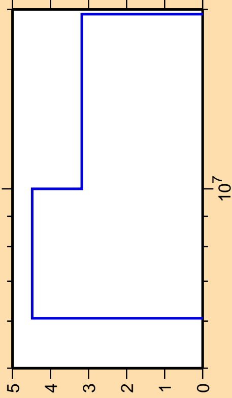
\Delta\sigma/\sigma vs. E for ^{102}\text{Ru}(n,2n)
