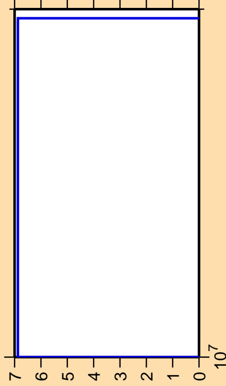
\Delta\sigma/\sigma vs. E for ^{102}\text{Ru}(n,\text{He3})
