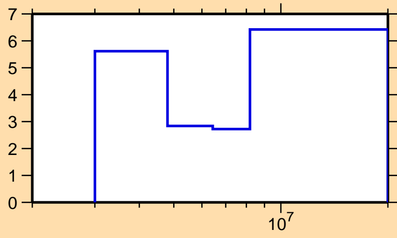
\Delta\sigma/\sigma vs. E for ^{102}\text{Ru}(n,n\text{cont.})
