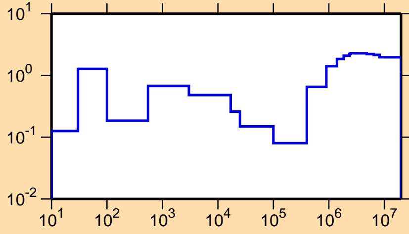
\sigma vs. E for ^{102}\text{Ru}(n,\text{nonel.})
