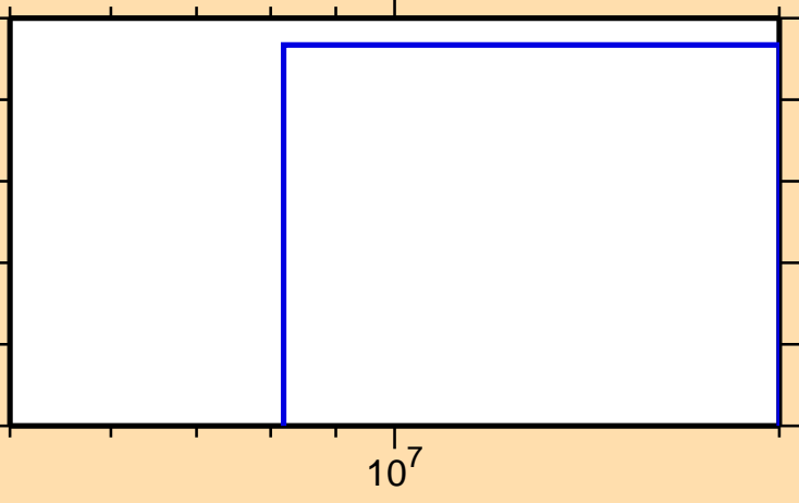
\sigma vs. E for ^{102}\text{Ru} (mt 34)
