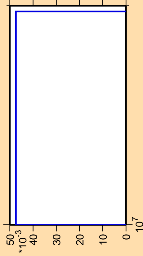
\Delta\sigma/\sigma vs. E for ^{103}\text{Ru}(n,p\alpha)
