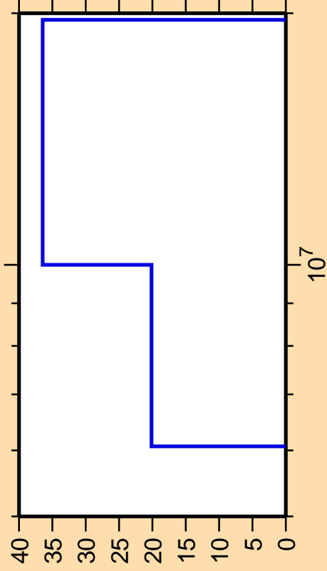
\Delta\sigma/\sigma vs. E for ^{103}\text{Ru}(n,\gamma)
