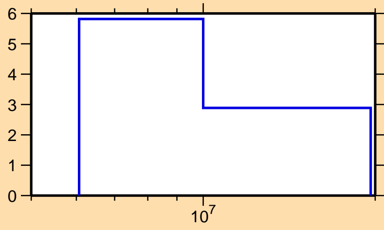
\Delta\sigma/\sigma vs. E for ^{103}\text{Ru}(n,2n)
