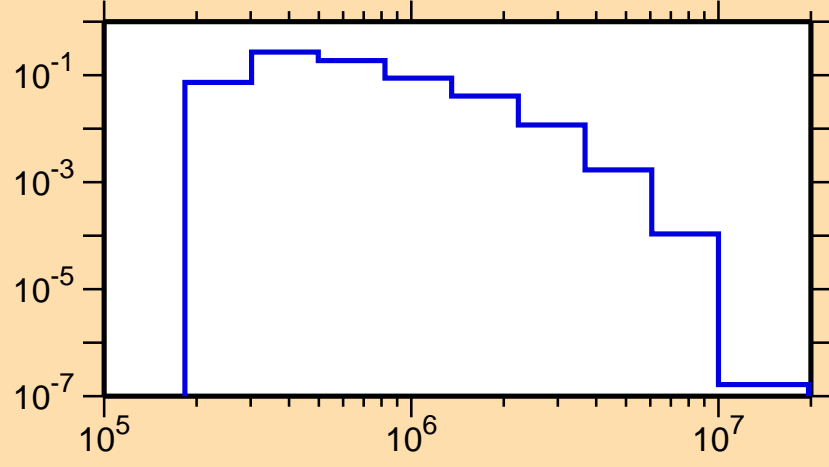
\sigma vs. E for ^{103}\text{Ru}(n,n_4)
