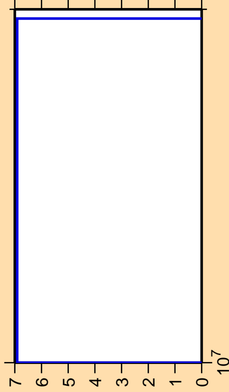
\Delta\sigma/\sigma vs. E for ^{103}\text{Ru}(n,3n)
