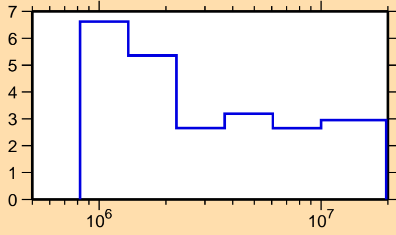
\Delta\sigma/\sigma vs. E for ^{103}\text{Ru}(n,\text{nonel.})
