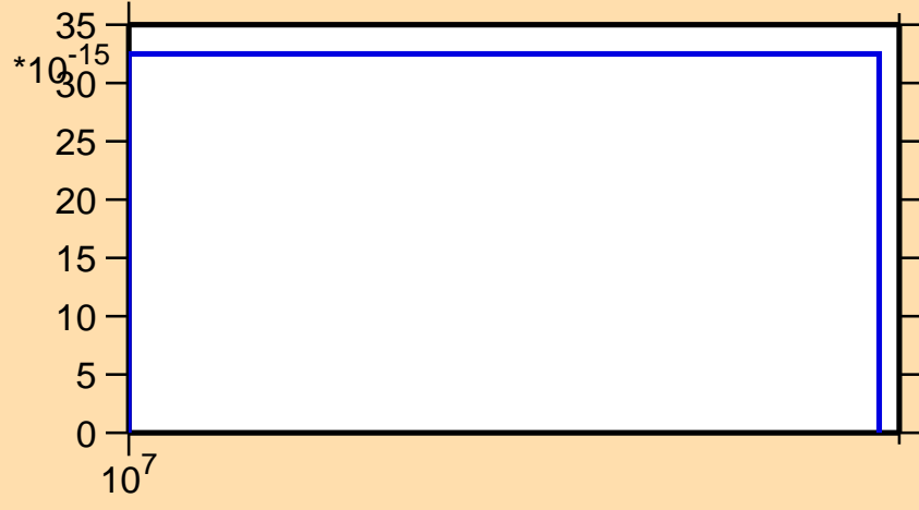
\sigma vs. E for ^{103}\text{Ru}(n,p\alpha)
