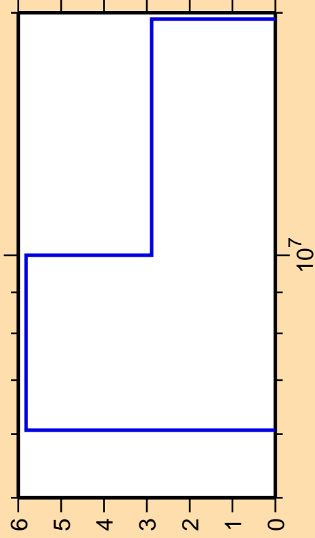
\Delta\sigma/\sigma vs. E for ^{103}\text{Ru}(n,2n)
