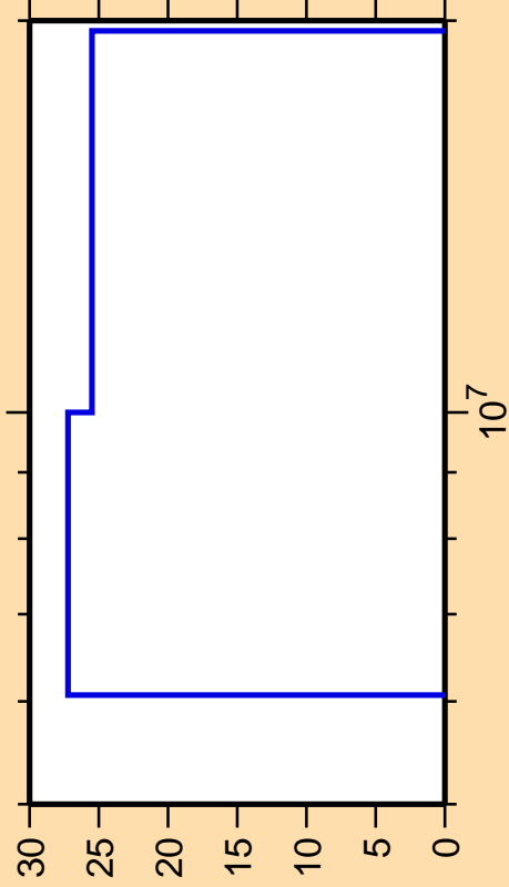
\Delta\sigma/\sigma vs. E for ^{103}\text{Ru}(n,p)
