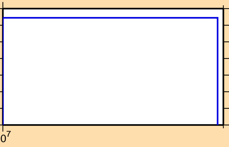
\sigma vs. E for ^{103}\text{Ru}(n,np)
