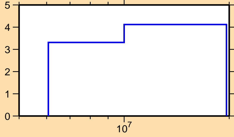
\Delta\sigma/\sigma vs. E for ^{103}\text{Ru}(n,\text{el.})
