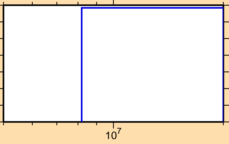
\sigma vs. E for ^{103}\text{Ru}(n,\text{nd})
