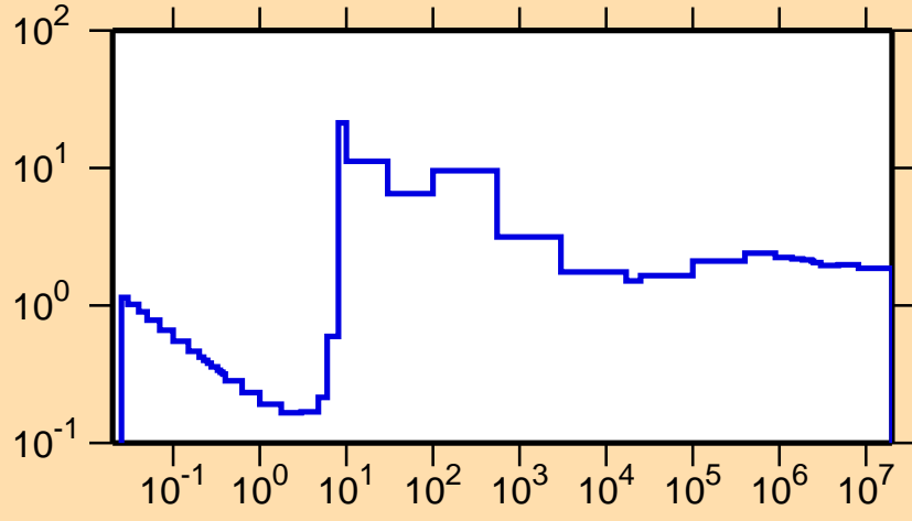
\sigma vs. E for ^{103}\text{Ru}(n,\text{nonel.})
