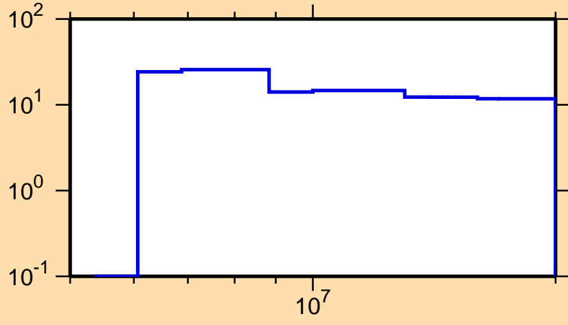
\Delta\sigma/\sigma vs. E for ^{104}\text{Ru}(n,p)
