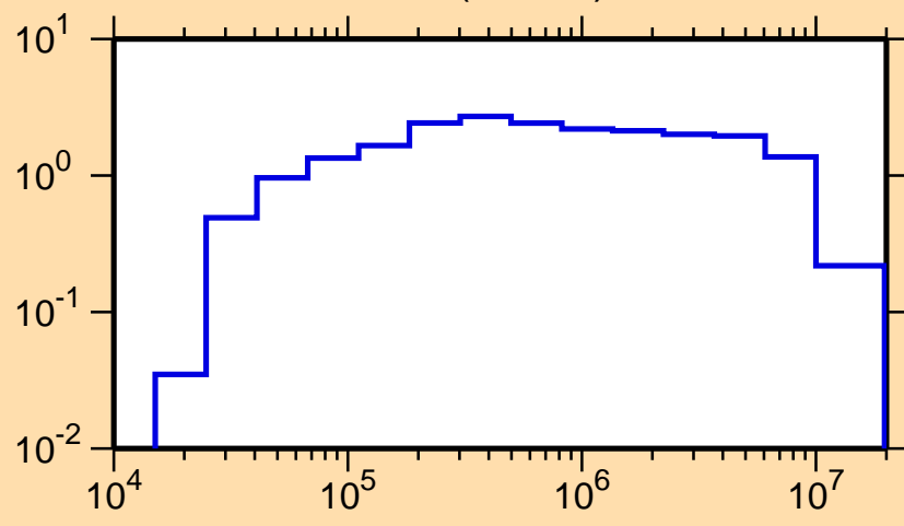
\sigma vs. E for ^{105}\text{Ru}(n,\text{inel.})
