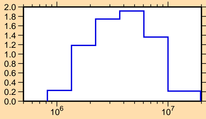
\sigma vs. E for ^{105}\text{Ru}(n,n\text{cont.})
