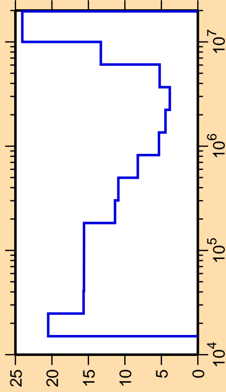
\Delta\sigma/\sigma vs. E for ^{105}\text{Ru}(n,\text{inel.})
