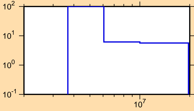
\Delta\sigma/\sigma vs. E for ^{105}\text{Ru}(n,2n)
