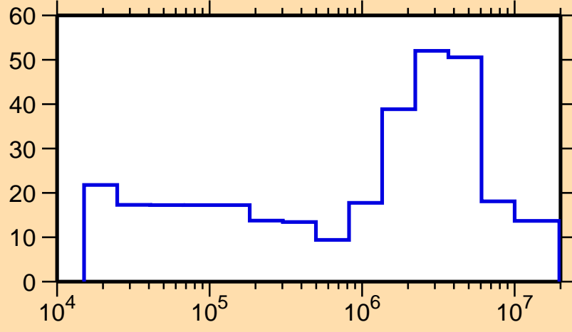
\Delta\sigma/\sigma vs. E for ^{105}\text{Ru}(n,n_1)
