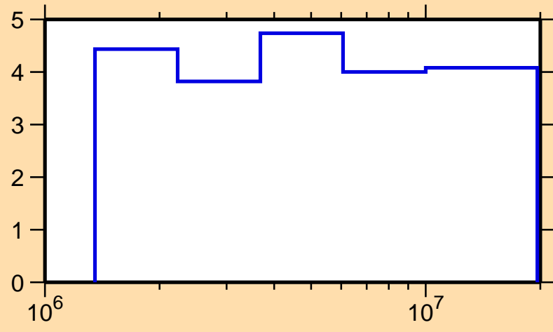
\Delta\sigma/\sigma vs. E for ^{105}\text{Ru}(n,\text{nonel.})
