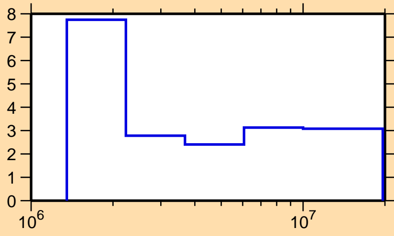
\Delta\sigma/\sigma vs. E for ^{105}\text{Ru}(n,\text{el.})
