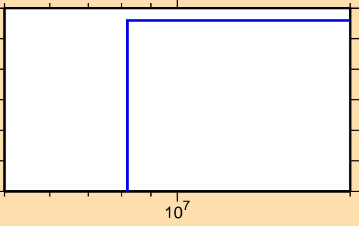
\sigma vs. E for ^{105}\text{Ru}(n,n\alpha)
