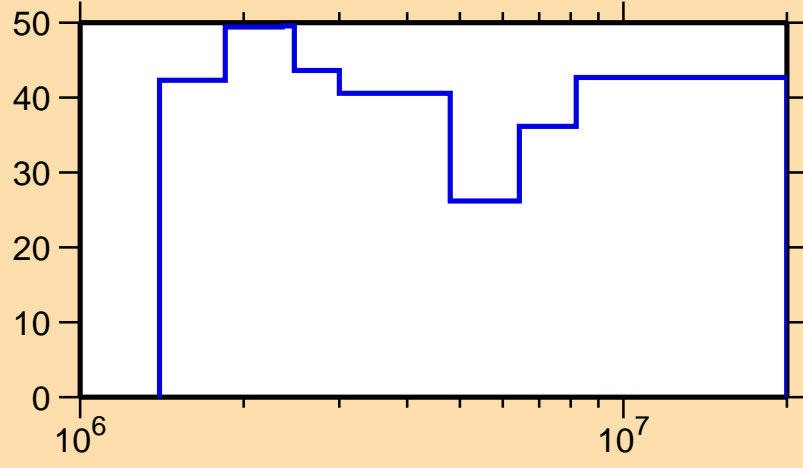
\Delta\sigma/\sigma vs. E for ^{105}\text{Ru}(n,\gamma)
