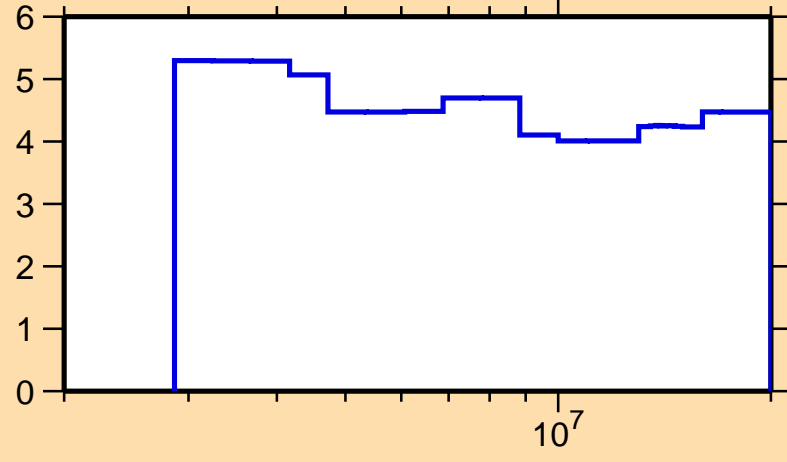
\Delta\sigma/\sigma vs. E for ^{106}\text{Ru}(n,n\text{onel.})
