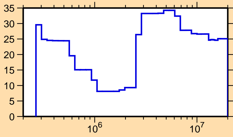
\Delta\sigma/\sigma vs. E for ^{106}\text{Ru}(n,n_1)
