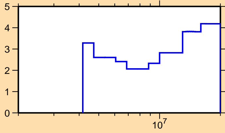
\Delta\sigma/\sigma vs. E for ^{106}\text{Ru}(n,\text{tot.})
