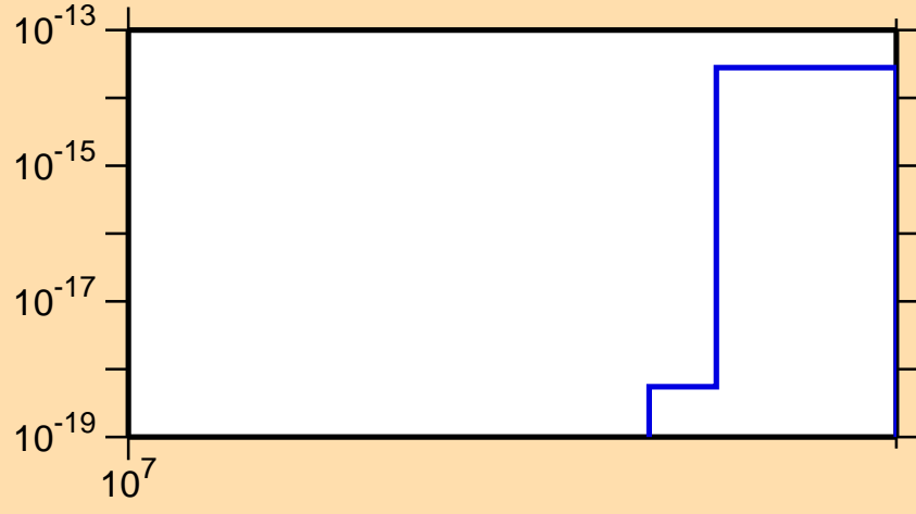
\sigma vs. E for ^{106}\text{Ru}(n,\text{He3})
