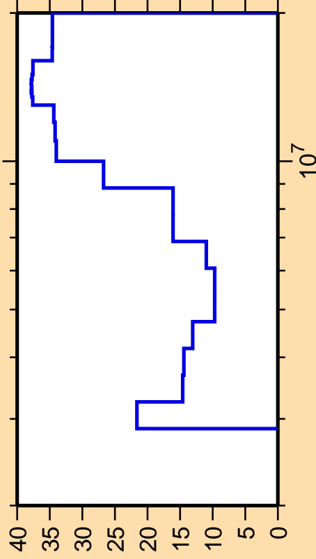
\Delta\sigma/\sigma vs. E for ^{106}\text{Ru}(n,n\text{cont.})
