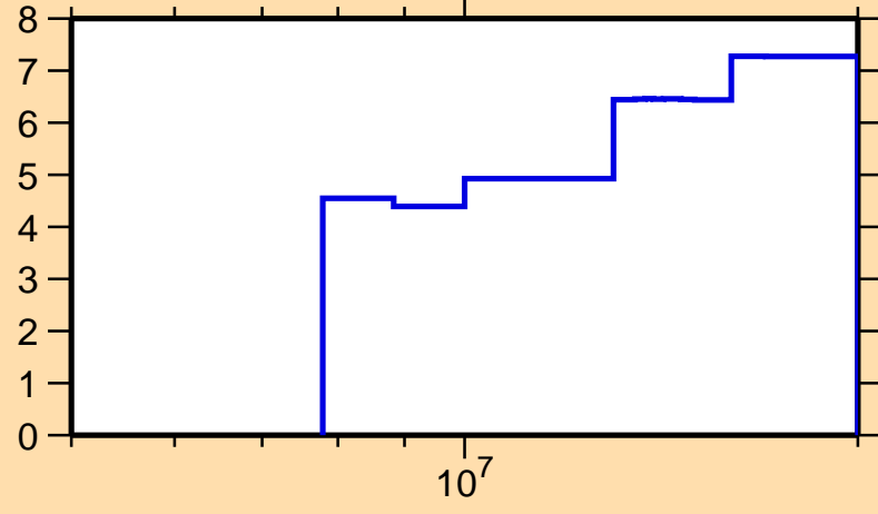
\Delta\sigma/\sigma vs. E for ^{106}\text{Ru}(n,\text{el.})
