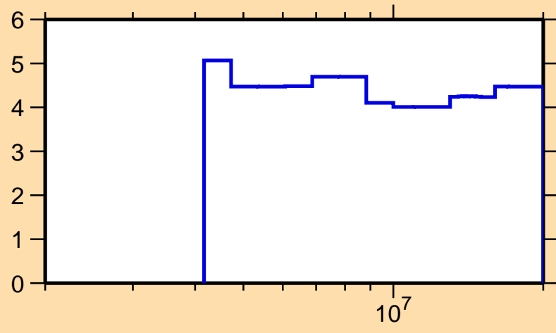
\Delta\sigma/\sigma vs. E for ^{106}\text{Ru}(n,\text{nonel.})
