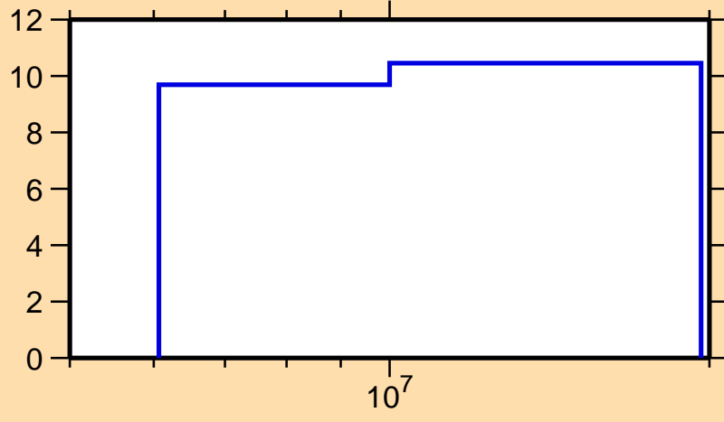
\Delta\sigma/\sigma vs. E for ^{106}\text{Ru}(n,2n)
