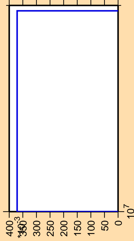
\Delta\sigma/\sigma vs. E for ^{106}\text{Ru}(n,nt)
