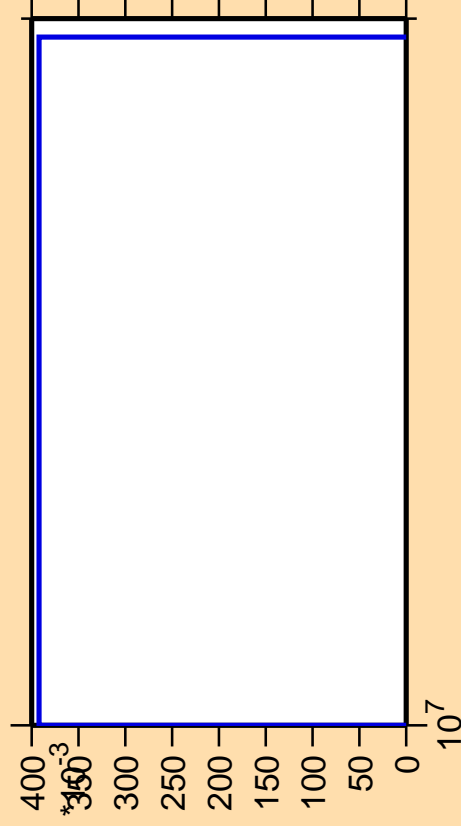
\Delta\sigma/\sigma vs. E for ^{106}\text{Ru}(n,\text{nd})
