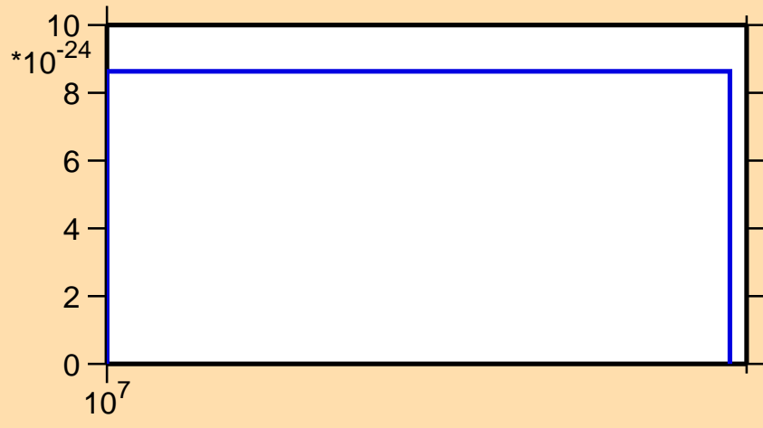
\sigma vs. E for ^{106}\text{Ru}(n,2np)
