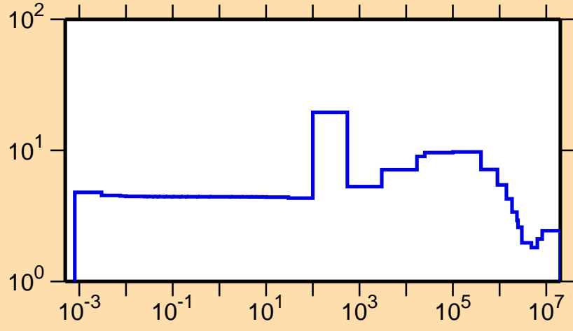
\sigma vs. E for ^{106}\text{Ru}(n,\text{el.})
