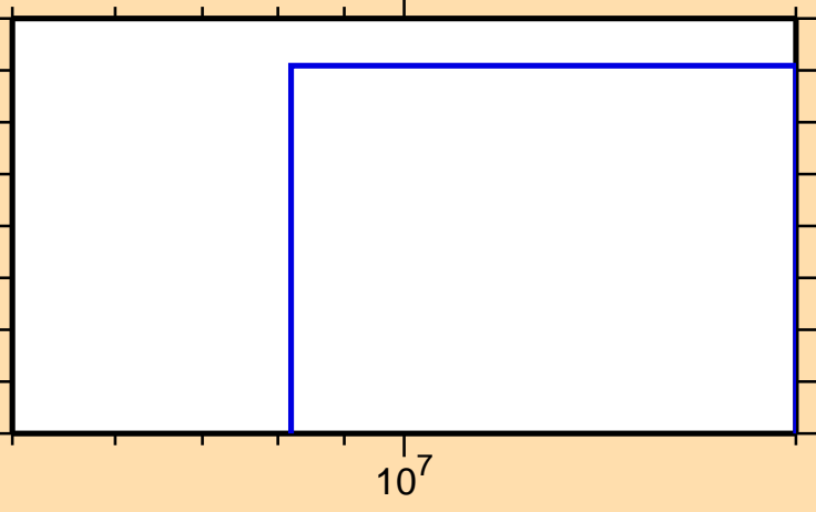
\sigma vs. E for ^{106}\text{Ru}(n,3n)
