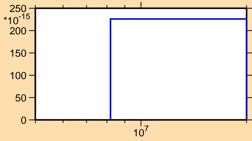
\sigma vs. E for ^{106}\text{Ru}(n,\text{nd})
