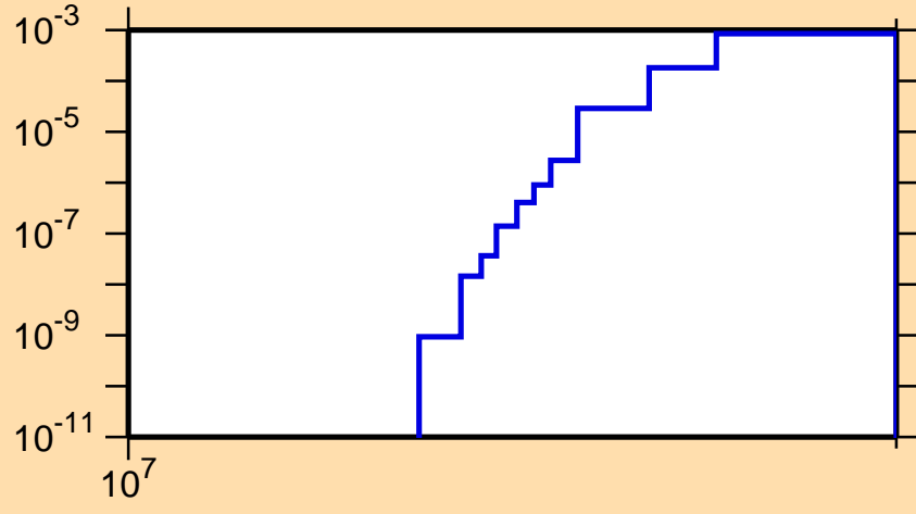
\sigma vs. E for ^{107}\text{Ru}(n,np)
