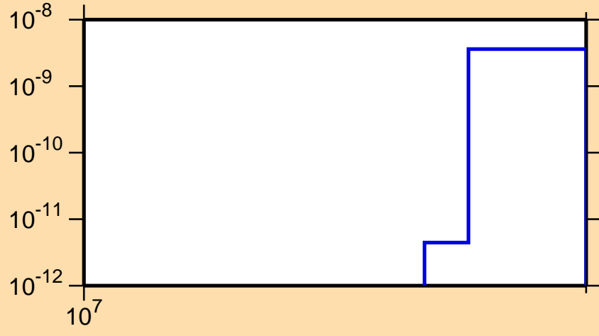
\sigma vs. E for ^{107}\text{Ru}(n,2n\alpha)
