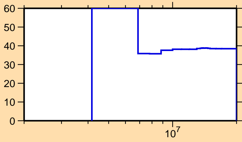
\Delta\sigma/\sigma vs. E for ^{107}\text{Ru}(n,\gamma)
