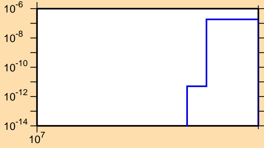
\sigma vs. E for ^{107}\text{Ru}(n,\text{nd})
