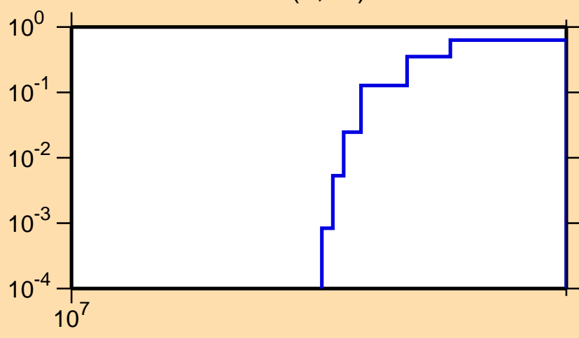
\sigma vs. E for ^{107}\text{Ru}(n,3n)
