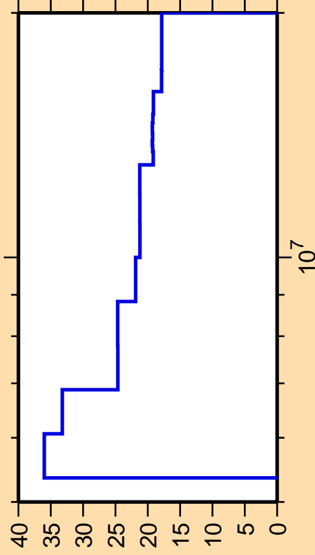
\Delta\sigma/\sigma vs. E for ^{107}\text{Ru}(n,n_1)
