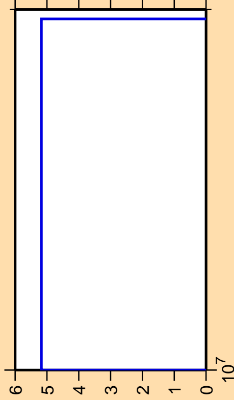
\Delta\sigma/\sigma vs. E for ^{107}\text{Ru}(n,nt)
