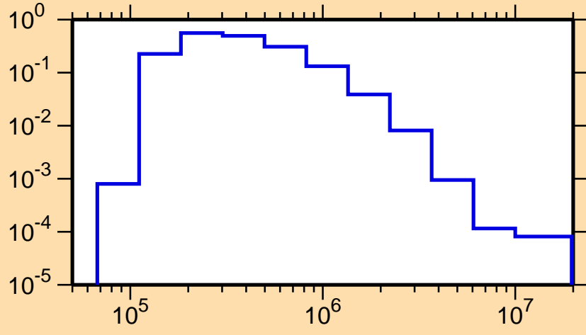
\sigma vs. E for ^{107}\text{Ru}(n,n_2)
