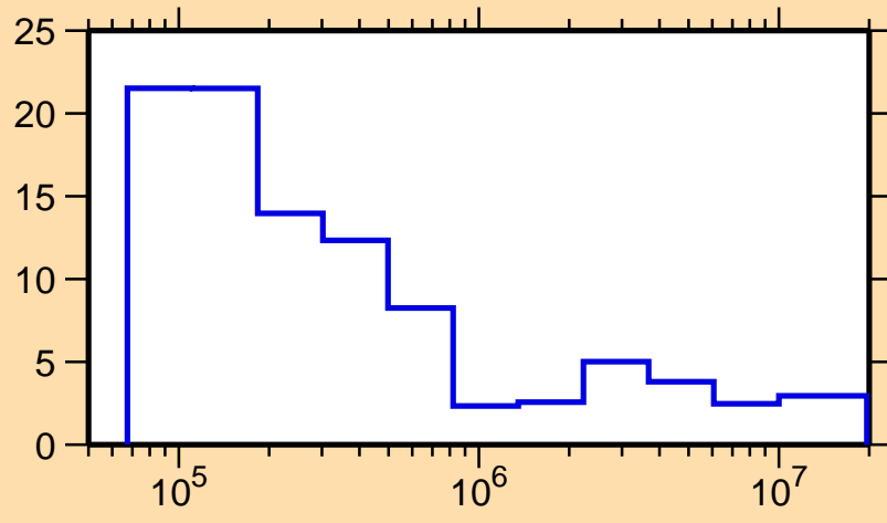
\Delta\sigma/\sigma vs. E for ^{107}\text{Ru}(n,\text{tot.})
