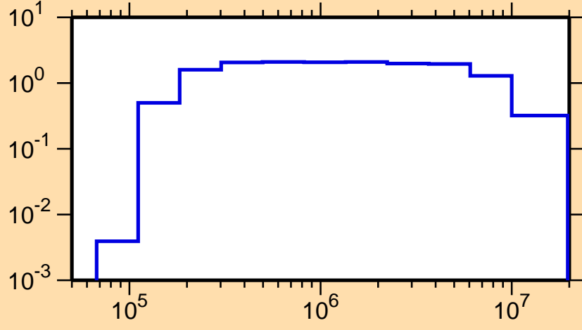
\sigma vs. E for ^{107}\text{Ru}(n,\text{inel.})
