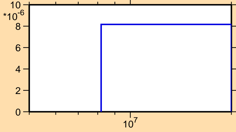
\sigma vs. E for ^{107}\text{Ru}(n,n\alpha)
