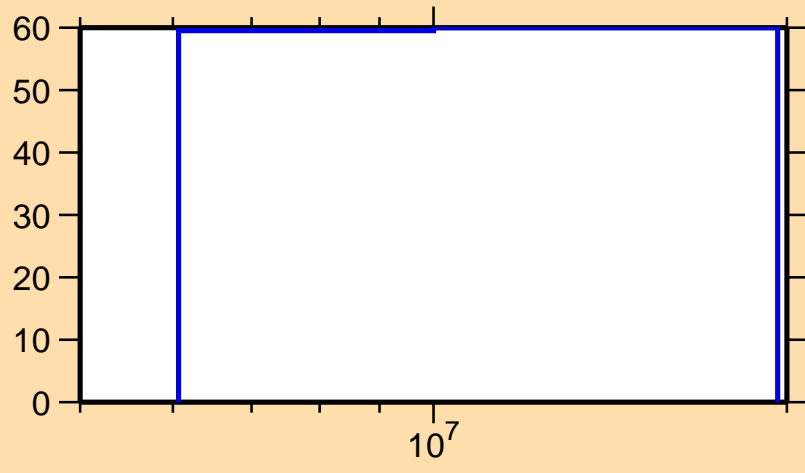
\Delta\sigma/\sigma vs. E for ^{108}\text{Ru}(n,p)
