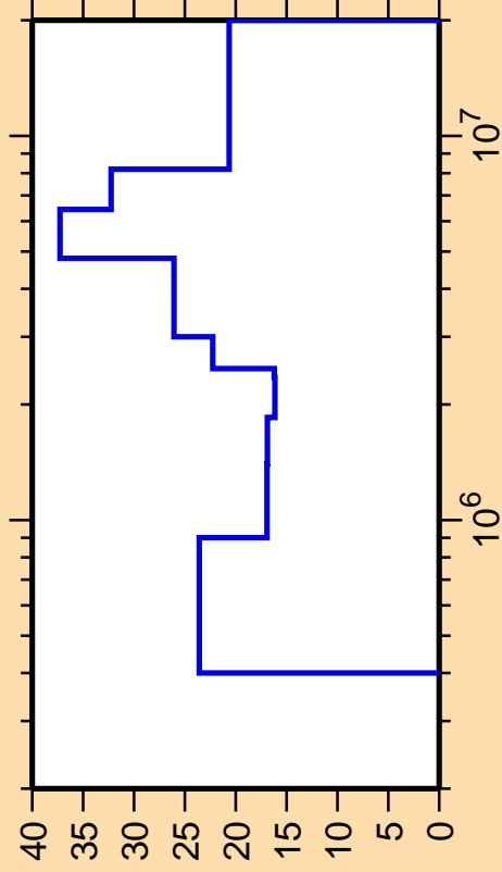
\Delta\sigma/\sigma vs. E for ^{108}\text{Ru}(n,n_3)
