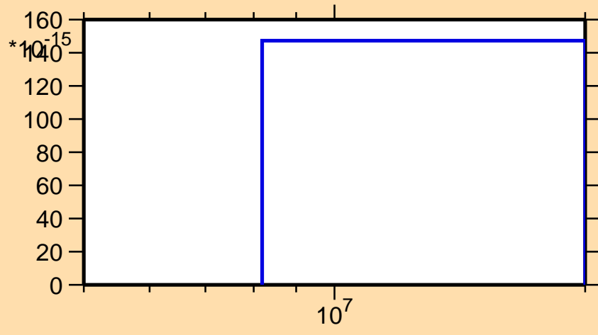
\sigma vs. E for ^{108}\text{Ru}(n,nd)
