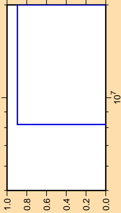
\Delta\sigma/\sigma vs. E for ^{108}\text{Ru}(n,nd)
