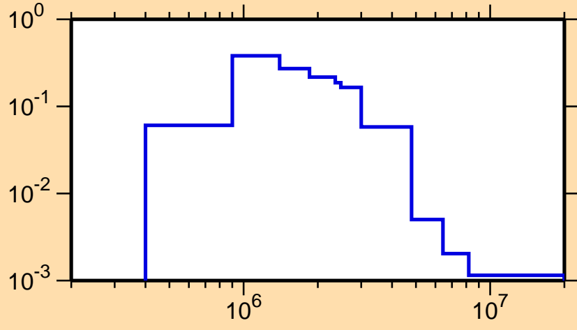
\sigma vs. E for ^{108}\text{Ru}(n,n_3)
