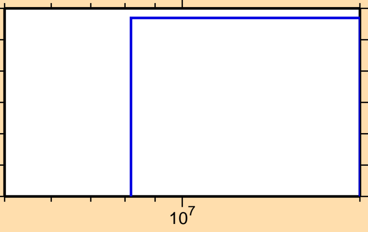
\sigma vs. E for ^{108}\text{Ru}(n,2np)
