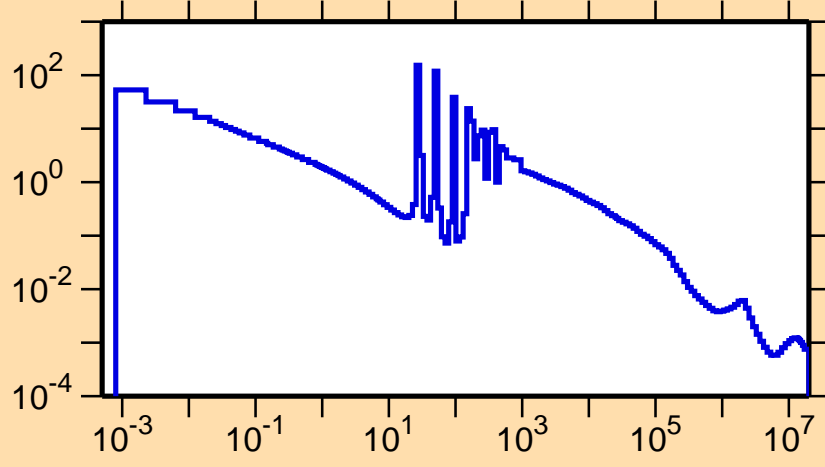
\sigma vs. E for ^{109}\text{Ru}(n,\gamma)
