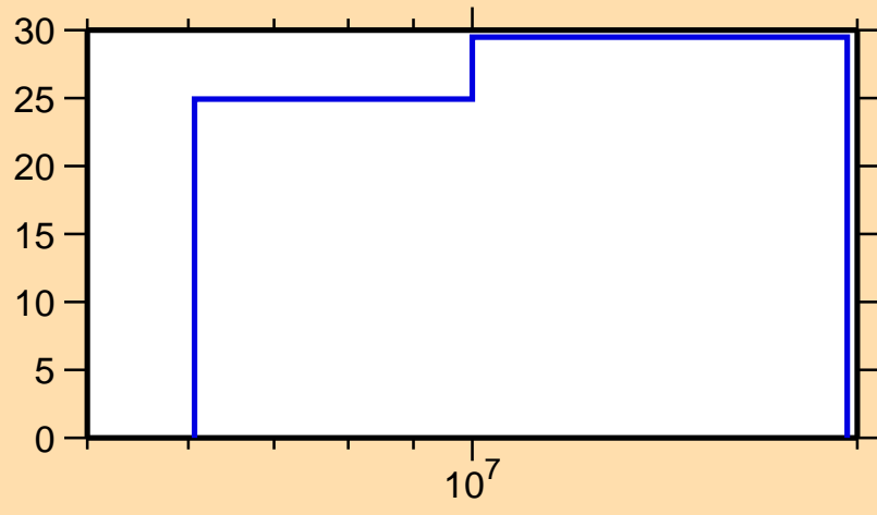
\Delta\sigma/\sigma vs. E for ^{109}\text{Ru}(n,p)
