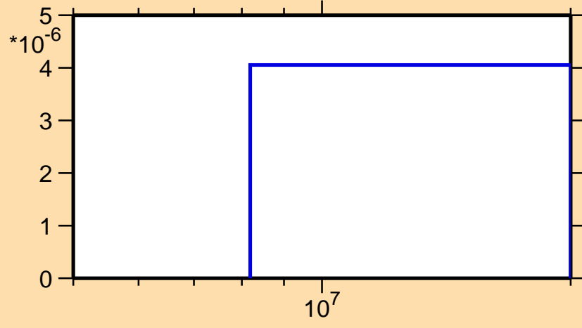
\sigma vs. E for ^{109}\text{Ru}(n,np)
