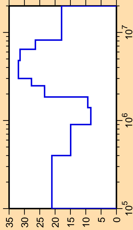
\Delta\sigma/\sigma vs. E for ^{109}\text{Ru}(n,n_4)
