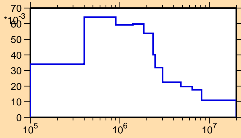
\sigma vs. E for ^{109}\text{Ru}(n,n_4)
