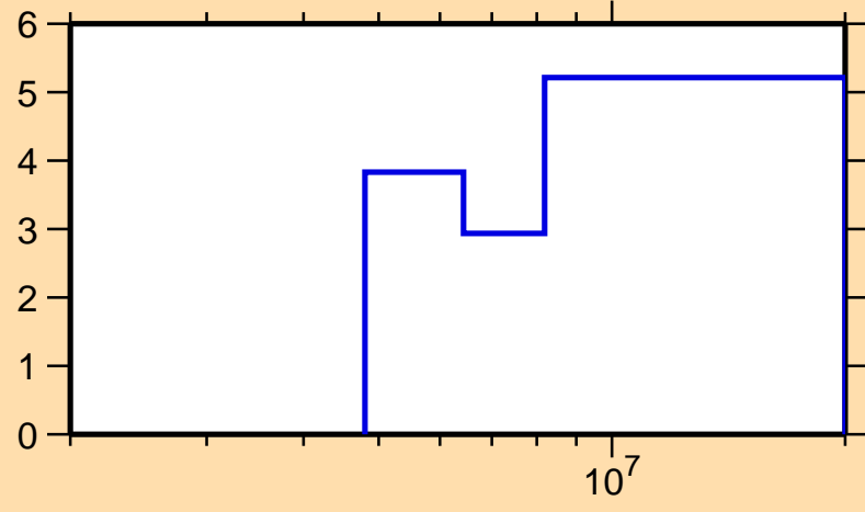
\Delta\sigma/\sigma vs. E for ^{109}\text{Ru}(n,\text{el.})
