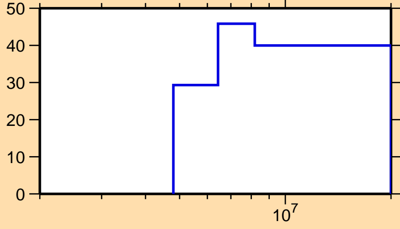
\Delta\sigma/\sigma vs. E for ^{109}\text{Ru}(n,n\text{cont.})
