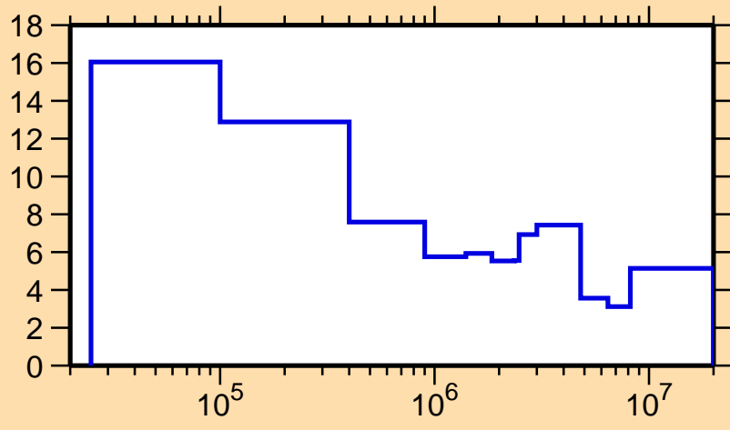
\Delta\sigma/\sigma vs. E for ^{109}\text{Ru}(n,\text{tot.})
