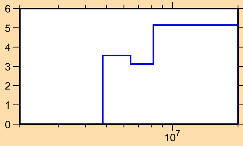
\Delta\sigma/\sigma vs. E for ^{109}\text{Ru}(n,\text{tot.})
