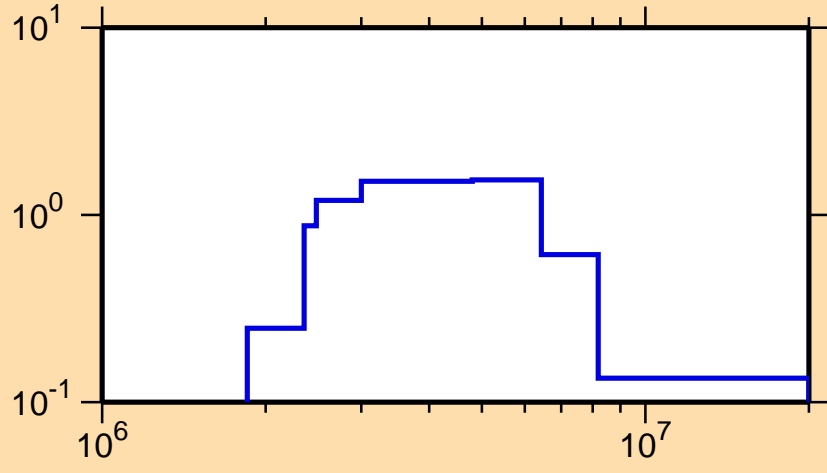
\sigma vs. E for ^{109}\text{Ru}(n,n\text{cont.})
