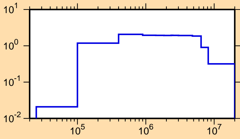
\sigma vs. E for ^{109}\text{Ru}(n,\text{inel.})
