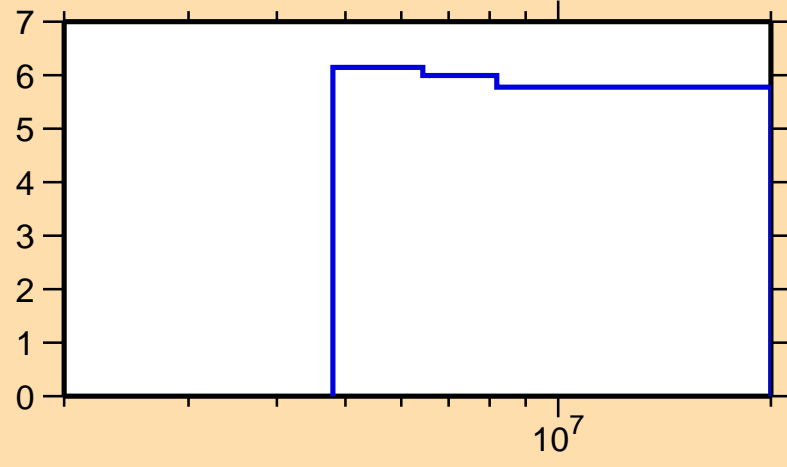
\Delta\sigma/\sigma vs. E for ^{109}\text{Ru}(n,\text{nonel.})
