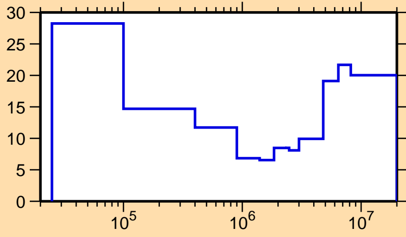
\Delta\sigma/\sigma vs. E for ^{109}\text{Ru}(n,\text{inel.})
