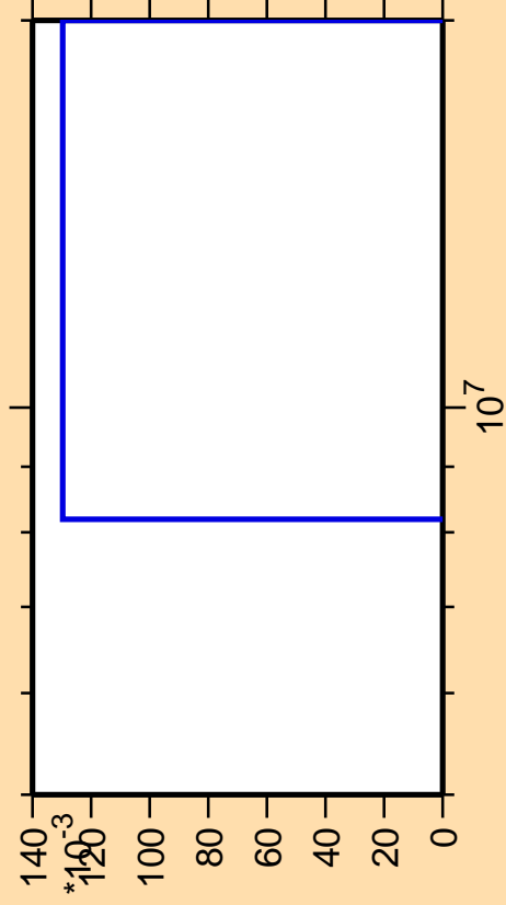
\Delta\sigma/\sigma vs. E for ^{109}\text{Ru}(n,2np)
