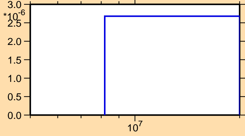
\sigma vs. E for ^{109}\text{Ru}(n,n\alpha)
