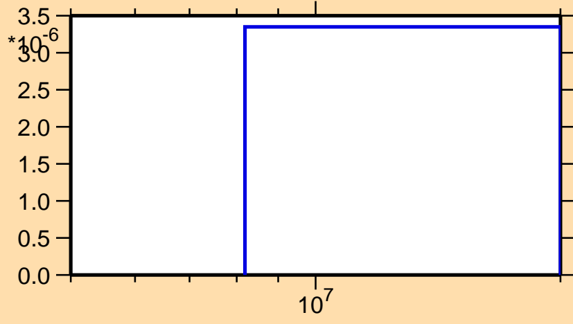
\sigma vs. E for ^{109}\text{Ru}(n,t)
