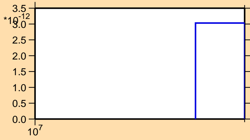
\sigma vs. E for ^{110}\text{Ru}(n,nd)
