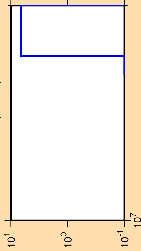
\Delta\sigma/\sigma vs. E for ^{110}\text{Ru}(n,2n\alpha)
