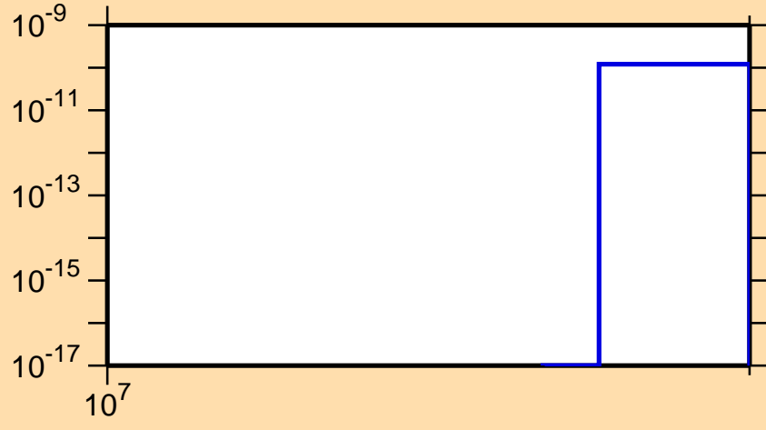
\sigma vs. E for ^{110}\text{Ru}(n,nt)
