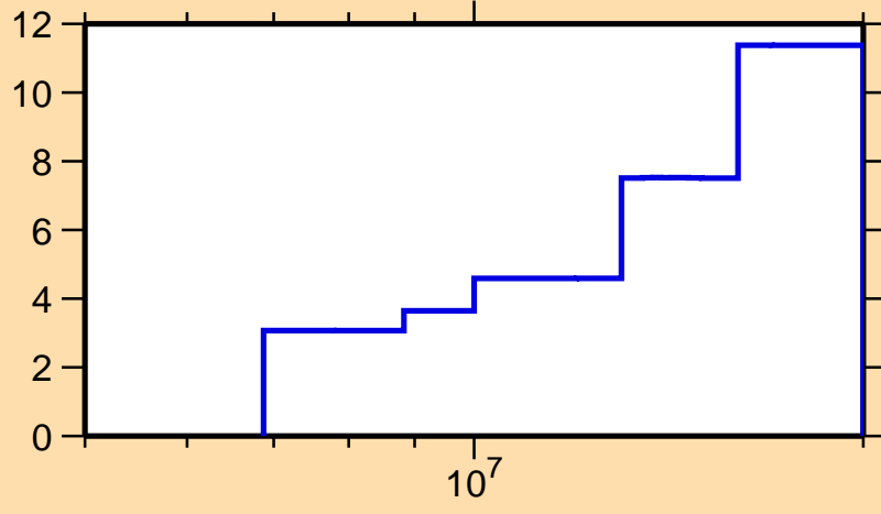
\Delta\sigma/\sigma vs. E for ^{110}\text{Ru}(n,\text{tot.})
