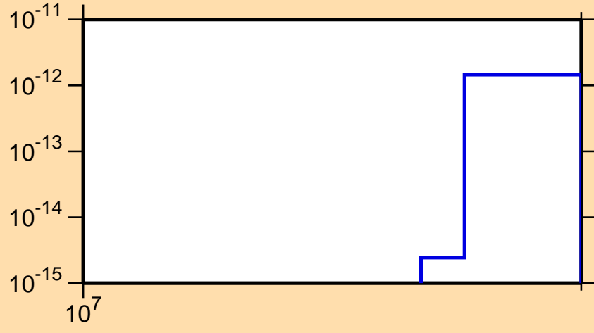
\sigma vs. E for ^{110}\text{Ru}(n,2n\alpha)
