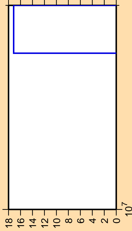
\Delta\sigma/\sigma vs. E for ^{110}\text{Ru}(n,nd)
