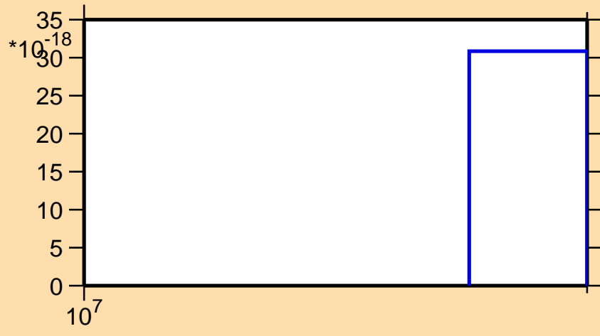
\sigma vs. E for ^{110}\text{Ru}(n,2np)
