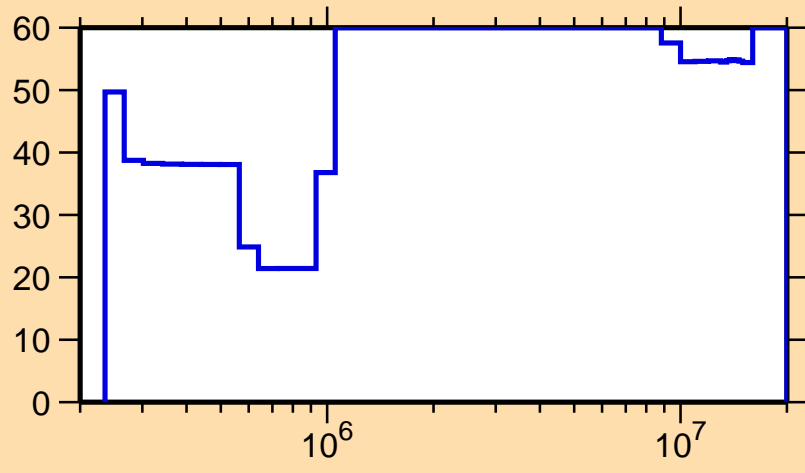
\Delta\sigma/\sigma vs. E for ^{110}\text{Ru}(n,n_1)
