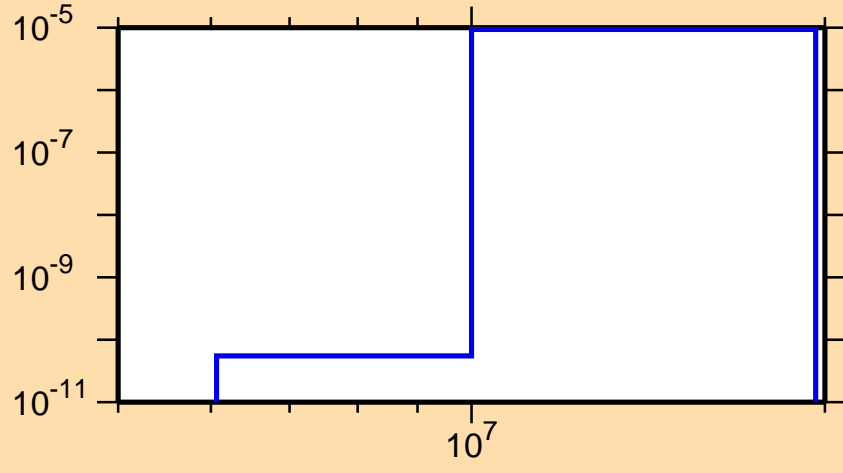
\sigma vs. E for ^{110}\text{Ru}(n,\alpha)
