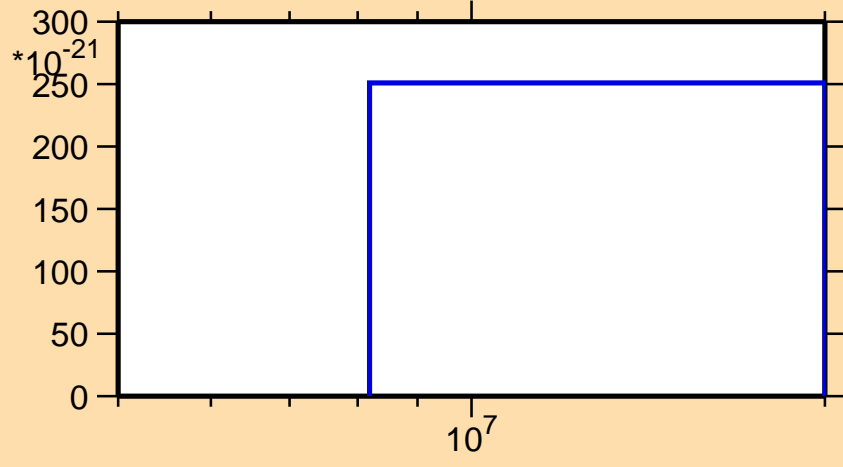
\sigma vs. E for ^{110}\text{Ru}(n,2np)
