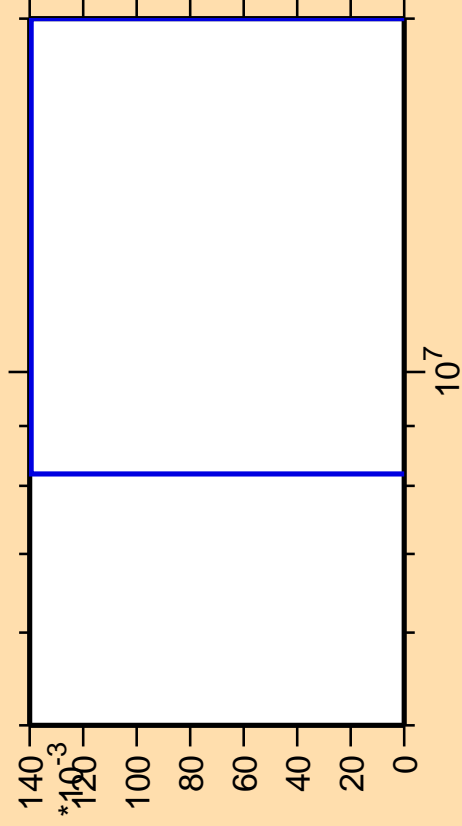
\Delta\sigma/\sigma vs. E for ^{110}\text{Ru}(n,nd)
