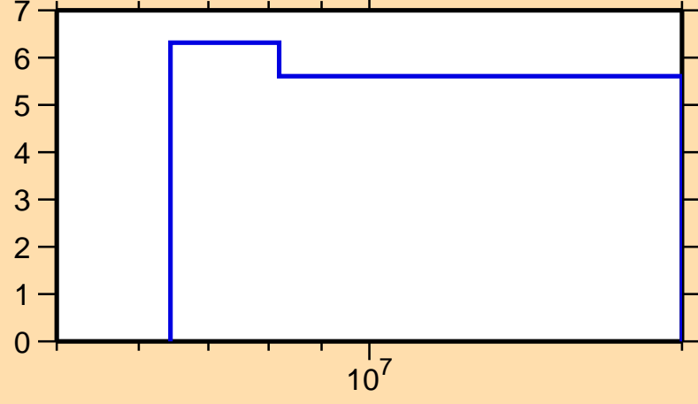
\Delta\sigma/\sigma vs. E for ^{110}\text{Ru}(n,\text{nonel.})
