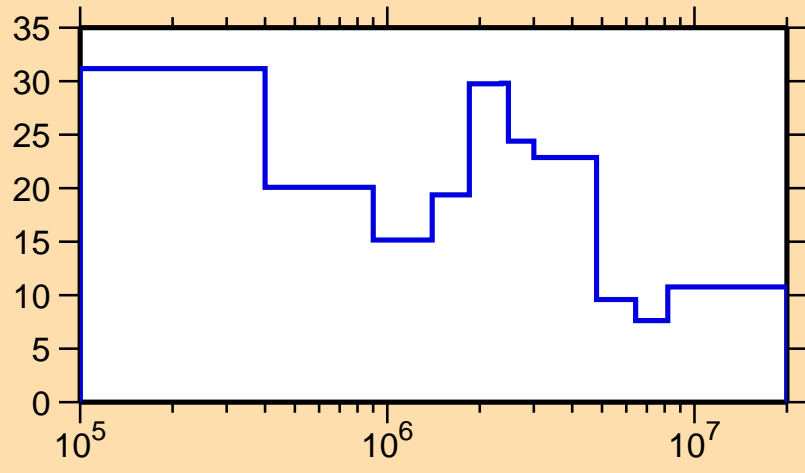
\Delta\sigma/\sigma vs. E for ^{110}\text{Ru}(n,\text{el.})
