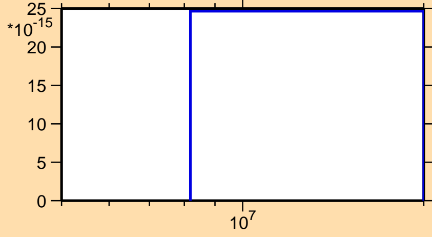
\sigma vs. E for ^{110}\text{Ru}(n,nd)
