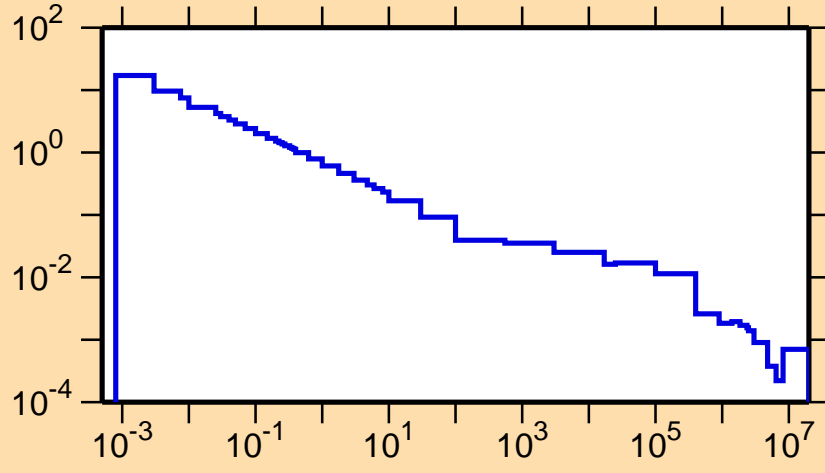
\sigma vs. E for ^{110}\text{Ru}(n,\gamma)
