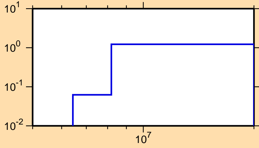
\sigma vs. E for ^{110}\text{Ru}(n,2n)
