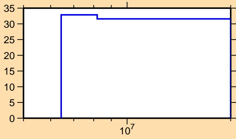
\Delta\sigma/\sigma vs. E for ^{110}\text{Ru}(n,\text{inel.})
