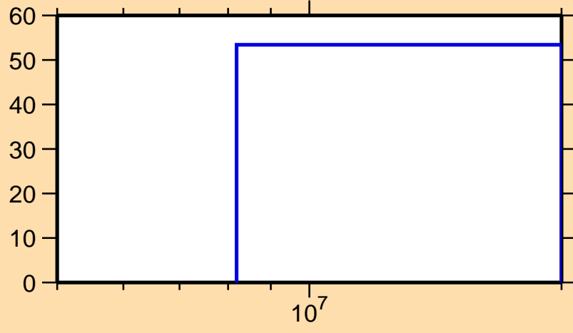
\Delta\sigma/\sigma vs. E for ^{110}\text{Ru}(n,ncont.)
