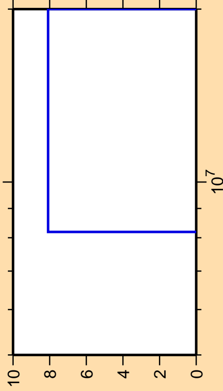
\Delta\sigma/\sigma vs. E for ^{110}\text{Ru}(n,nt)
