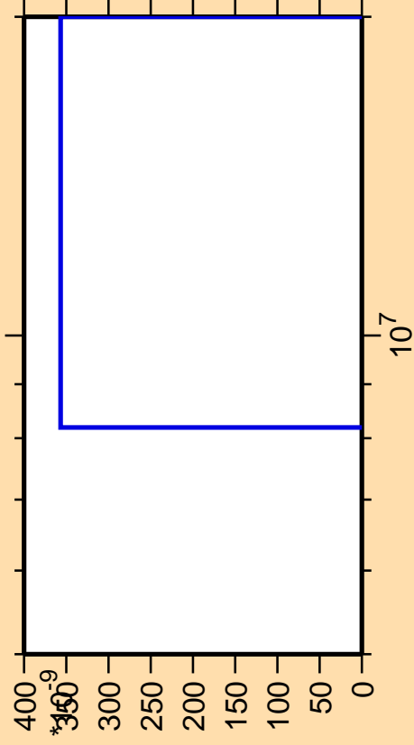
\Delta\sigma/\sigma vs. E for ^{110}\text{Ru}(n,2np)
