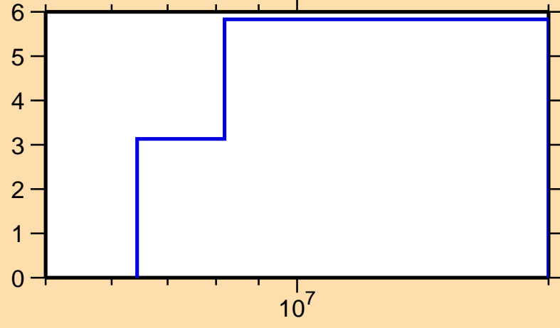
\Delta\sigma/\sigma vs. E for ^{110}\text{Ru}(n,\text{tot.})
