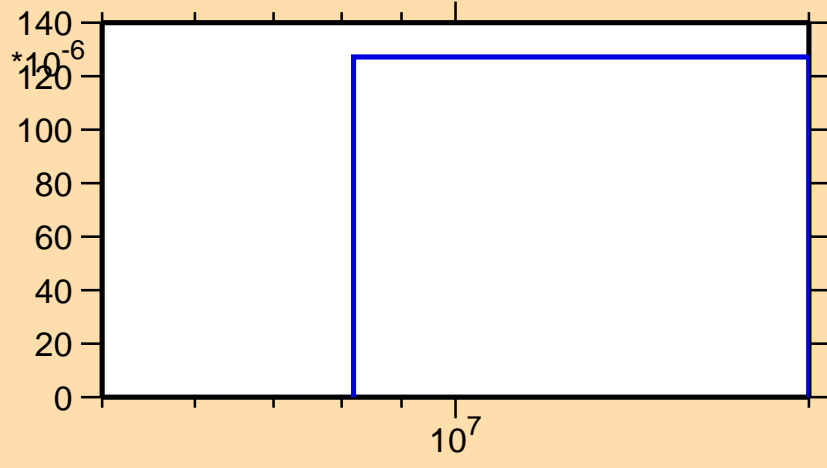
\sigma vs. E for ^{110}\text{Ru}(n,p)
