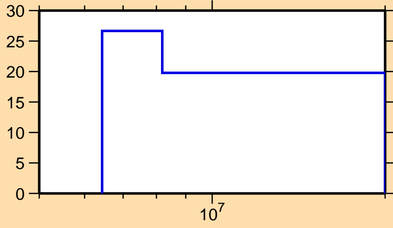
\Delta\sigma/\sigma vs. E for ^{110}\text{Ru}(n,2n)
