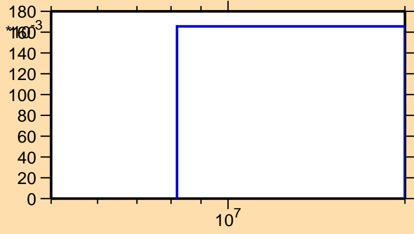
\sigma vs. E for ^{110}\text{Ru}(n,3n)
