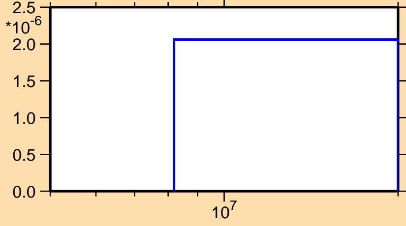
\sigma vs. E for ^{110}\text{Ru}(n,d)
