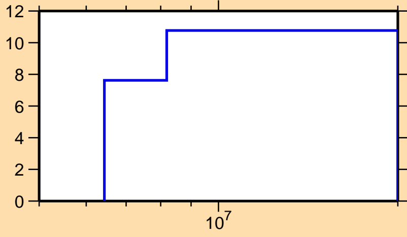
\Delta\sigma/\sigma vs. E for ^{110}\text{Ru}(n,\text{el.})
