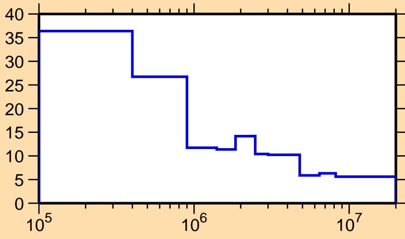
\Delta\sigma/\sigma vs. E for ^{110}\text{Ru}(n,\text{nonel.})
