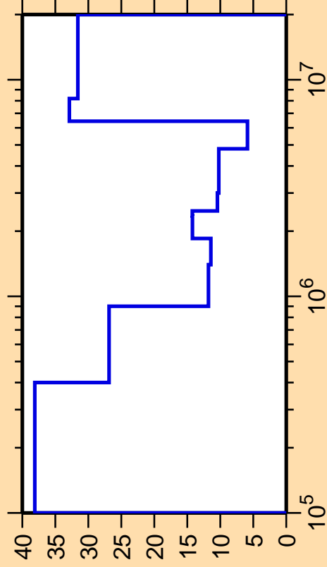
\Delta\sigma/\sigma vs. E for ^{110}\text{Ru}(n,\text{inel.})
