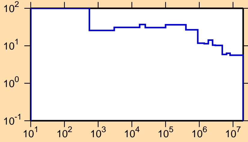
\Delta\sigma/\sigma vs. E for ^{110}\text{Ru}(n,\text{nonel.})
