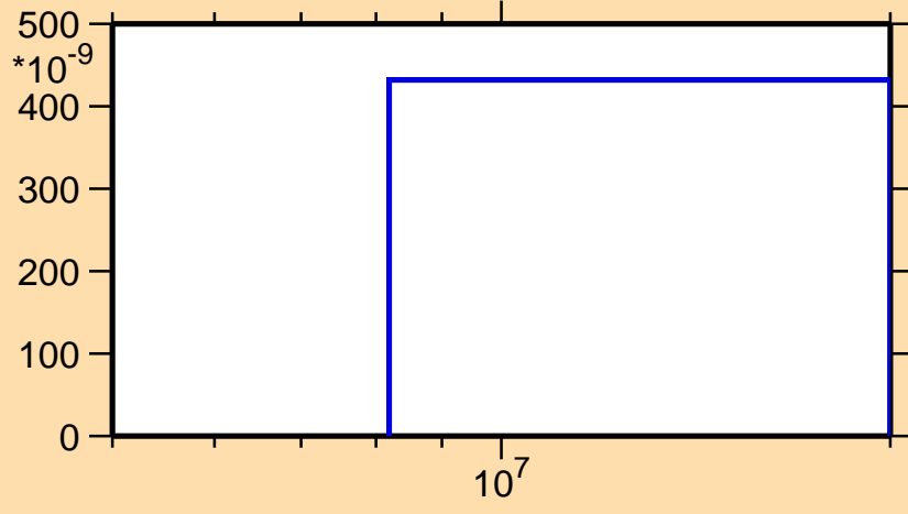
\sigma vs. E for ^{110}\text{Ru}(n,t)
