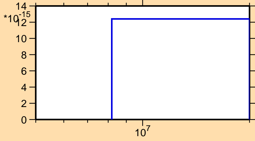
\sigma vs. E for ^{110}\text{Ru}(n,2n\alpha)
