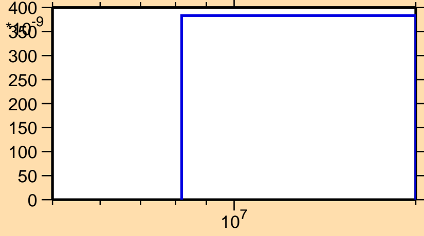
\sigma vs. E for ^{110}\text{Ru}(n,n\alpha)
