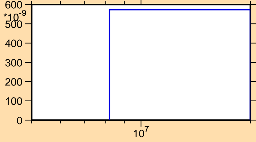
\sigma vs. E for ^{110}\text{Ru}(n,np)
