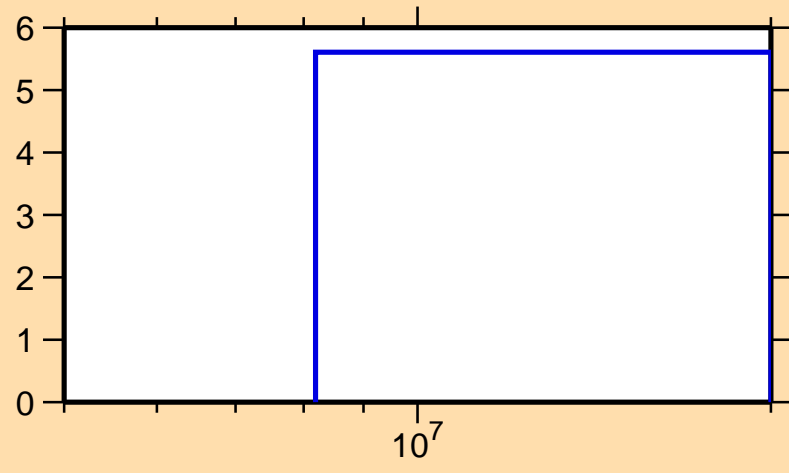
\Delta\sigma/\sigma vs. E for ^{110}\text{Ru}(n,\text{nonel.})
