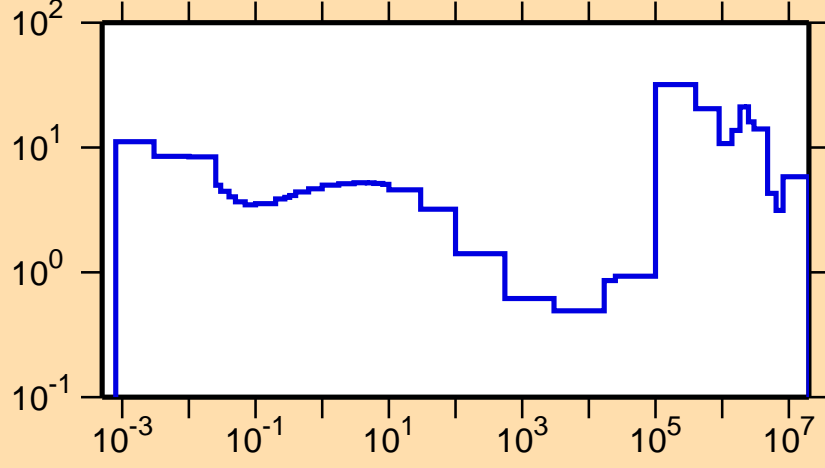
\Delta\sigma/\sigma vs. E for ^{110}\text{Ru}(n,\text{tot.})
