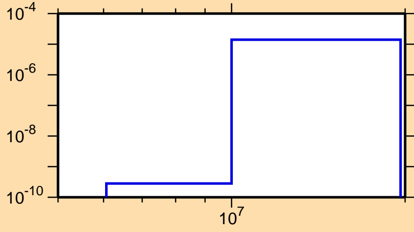
\sigma vs. E for ^{111}\text{Ru}(n,\alpha)
