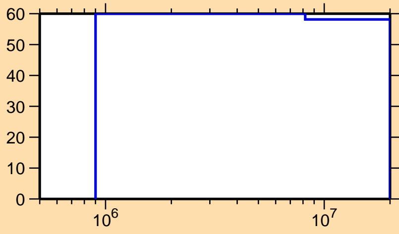
\Delta\sigma/\sigma vs. E for ^{111}\text{Ru}(n,n_1)
