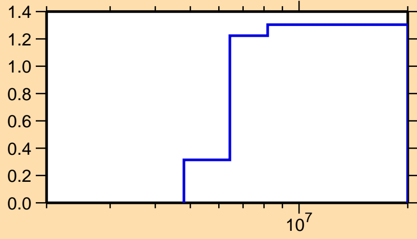
\sigma vs. E for ^{111}\text{Ru}(n,2n)
