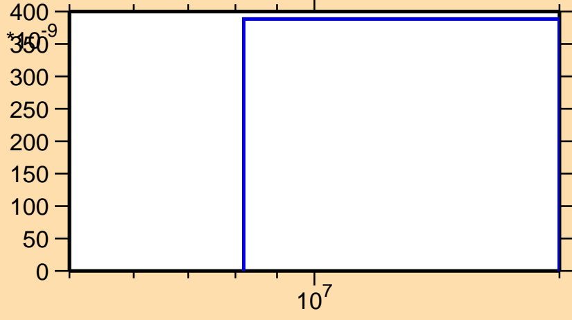
\sigma vs. E for ^{111}\text{Ru}(n,n\alpha)
