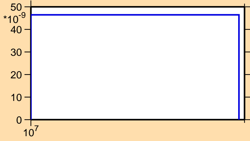
\sigma vs. E for ^{112}\text{Ru}(n,n\alpha)
