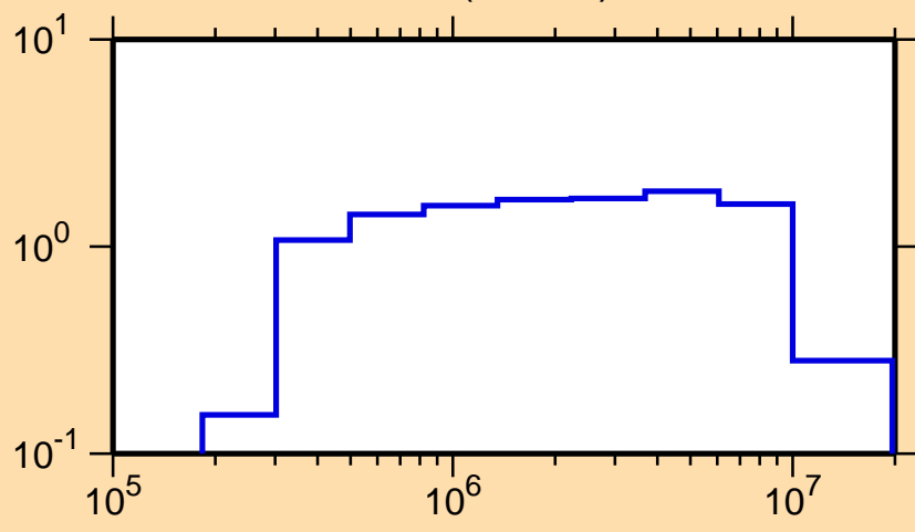
\sigma vs. E for ^{112}\text{Ru}(n,\text{inel.})
