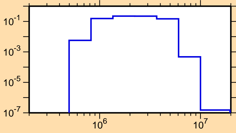
\sigma vs. E for ^{112}\text{Ru}(n,n_4)
