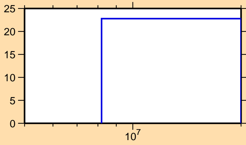
\Delta\sigma/\sigma vs. E for ^{112}\text{Ru}(n,ncont.)
