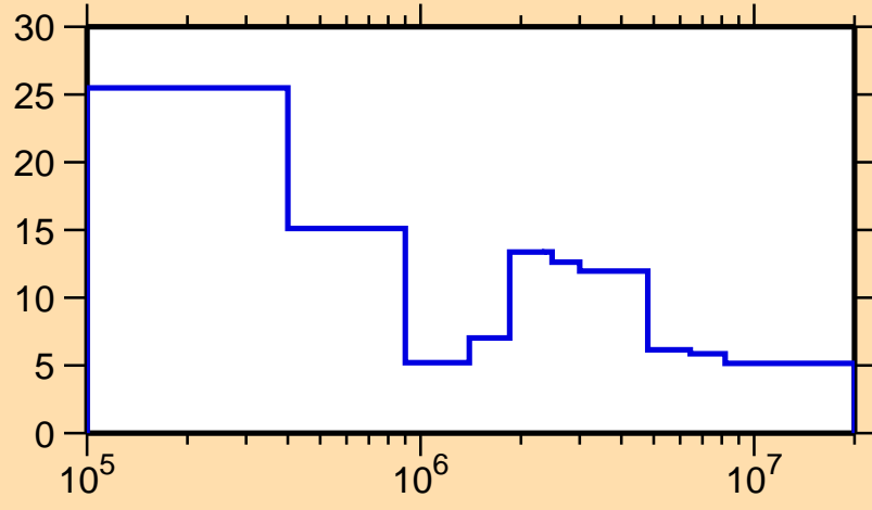
\Delta\sigma/\sigma vs. E for ^{112}\text{Ru}(n,\text{tot.})
