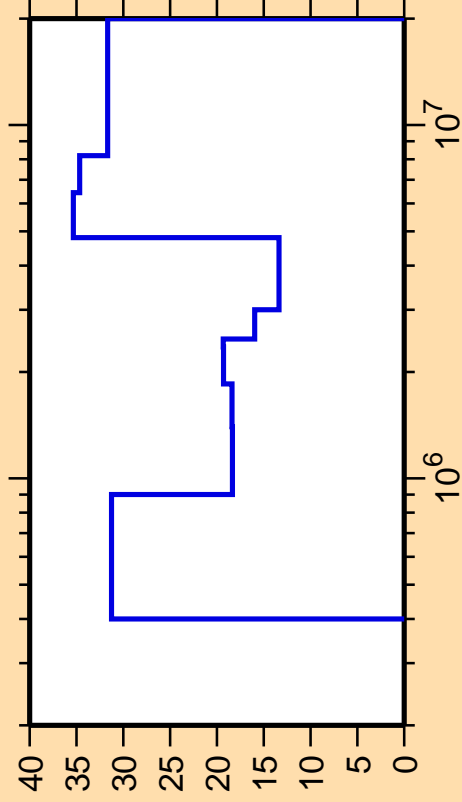
\Delta\sigma/\sigma vs. E for ^{112}\text{Ru}(n,n_3)
