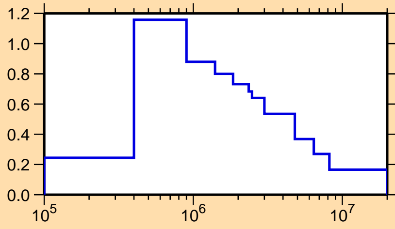
\sigma vs. E for ^{112}\text{Ru}(n,n_1)
