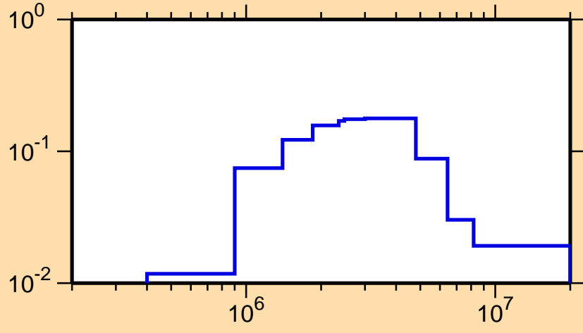
\sigma vs. E for ^{112}\text{Ru}(n,n_3)
