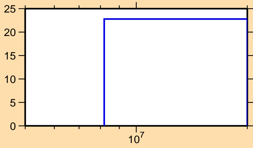
\Delta\sigma/\sigma vs. E for ^{112}\text{Ru}(n,n\text{cont.})
