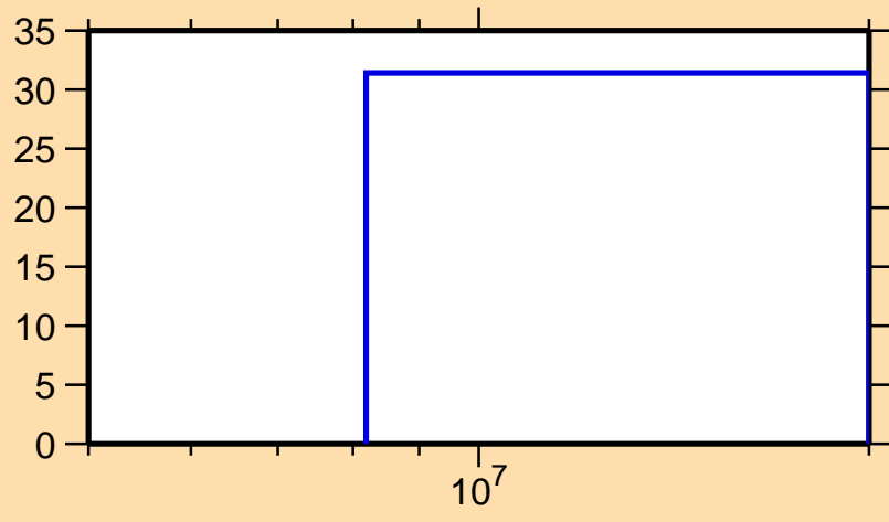
\Delta\sigma/\sigma vs. E for ^{112}\text{Ru}(n,n_1)
