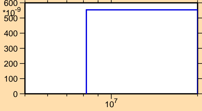
\sigma vs. E for ^{112}\text{Ru}(n,d)
