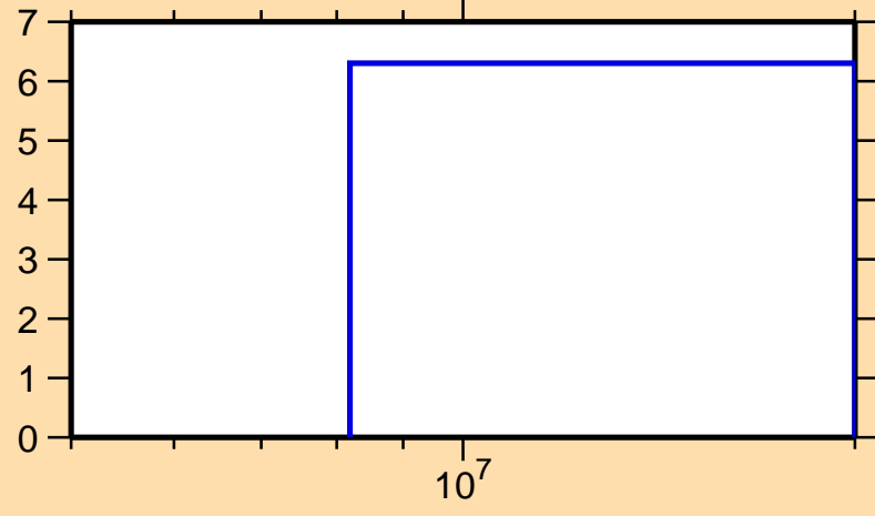
\Delta\sigma/\sigma vs. E for ^{112}\text{Ru}(n,\text{el.})
