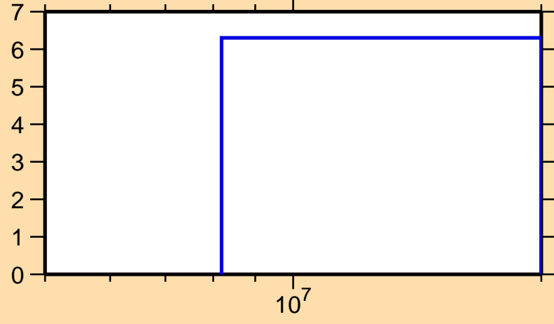
\Delta\sigma/\sigma vs. E for ^{112}\text{Ru}(n,el.)
