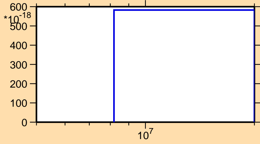
\sigma vs. E for ^{112}\text{Ru}(n,nd)
