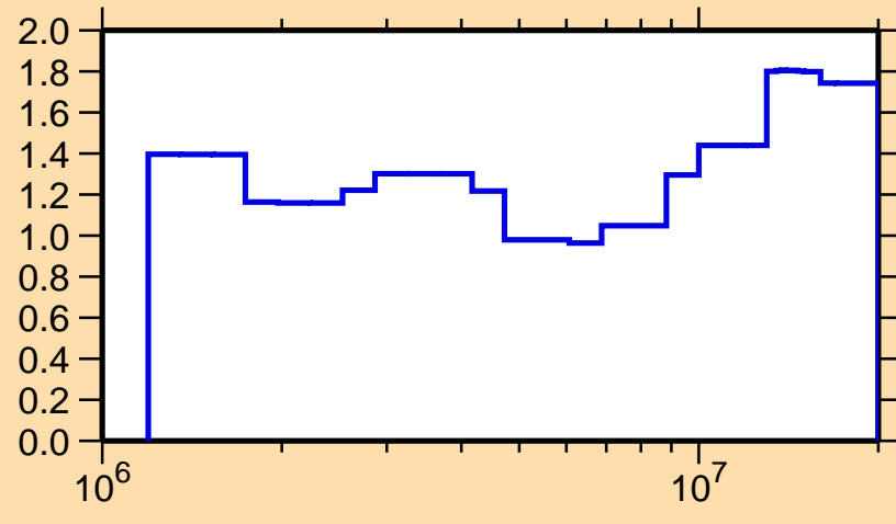
\Delta\sigma/\sigma vs. E for ^{31}\text{S}(n,\text{tot.})
