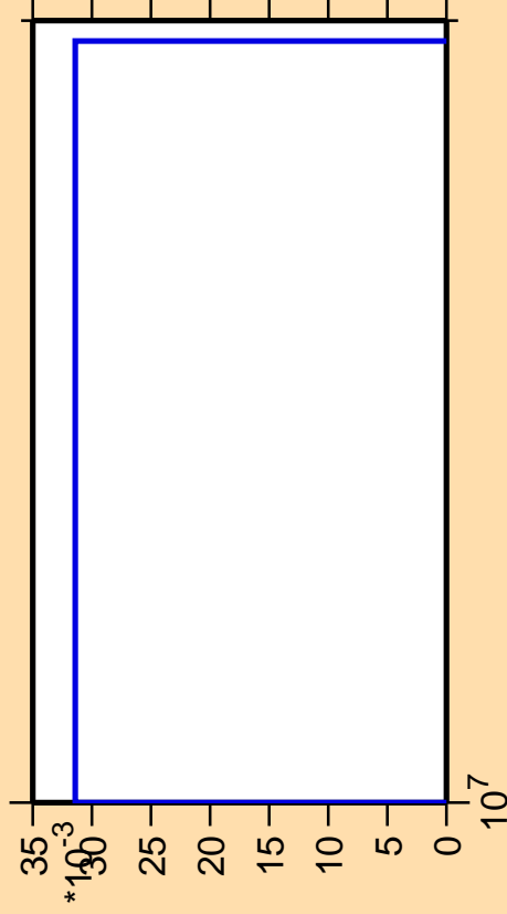
\Delta\sigma/\sigma vs. E for ^{32}\text{S}(\text{mt117})
