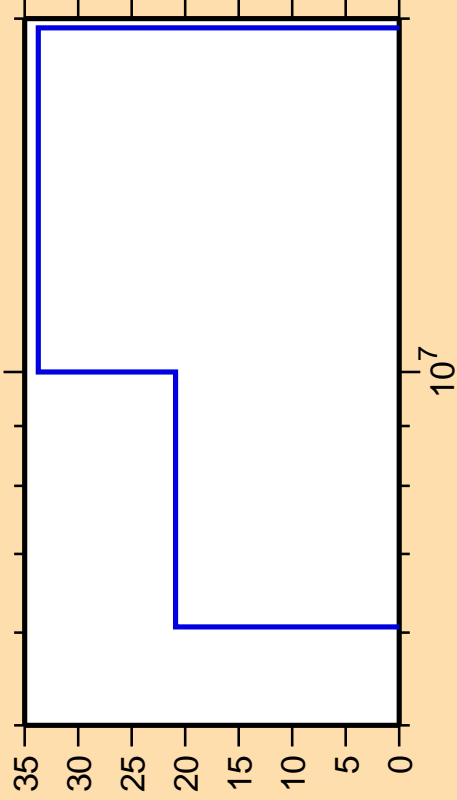
\Delta\sigma/\sigma vs. E for ^{32}\text{S}(n,d)
