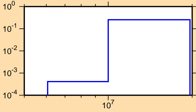
\sigma vs. E for ^{32}\text{S}(n,n\alpha)
