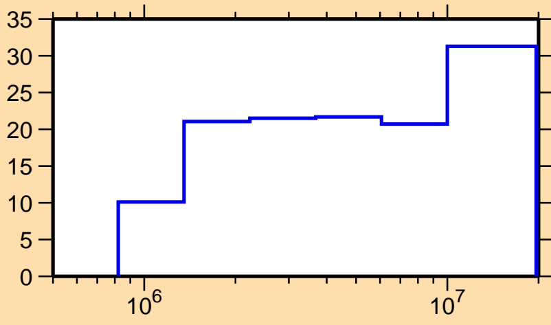
\Delta\sigma/\sigma vs. E for ^{32}\text{S}(n,\gamma)
