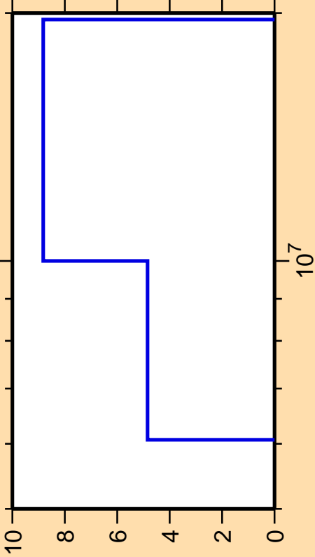
\Delta\sigma/\sigma vs. E for ^{32}\text{S}(n,p)
