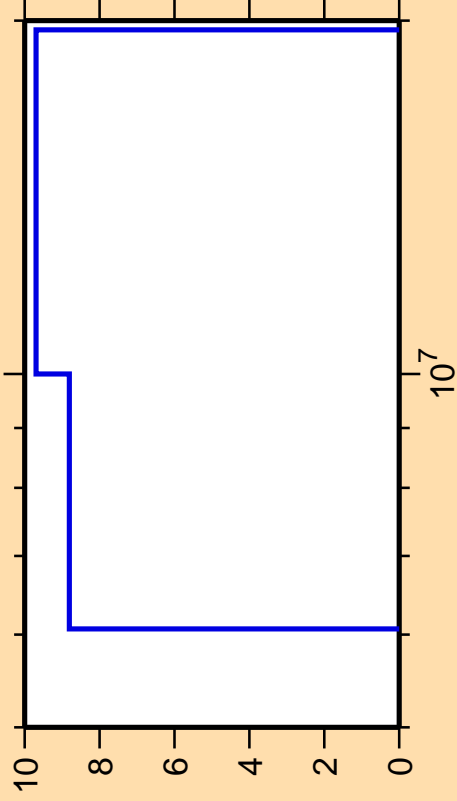
\Delta\sigma/\sigma vs. E for ^{32}\text{S}(n,\text{ncont.})
