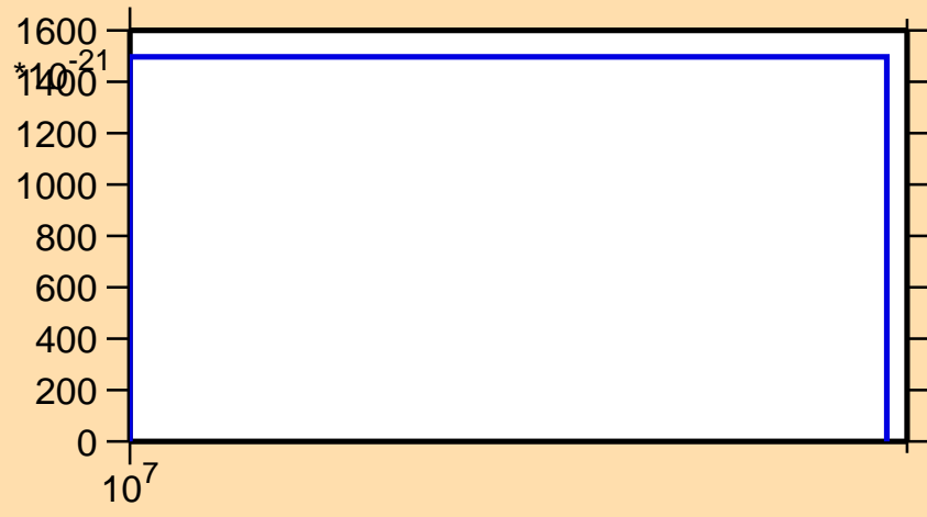
\sigma vs. E for ^{32}\text{S}(n,nd)
