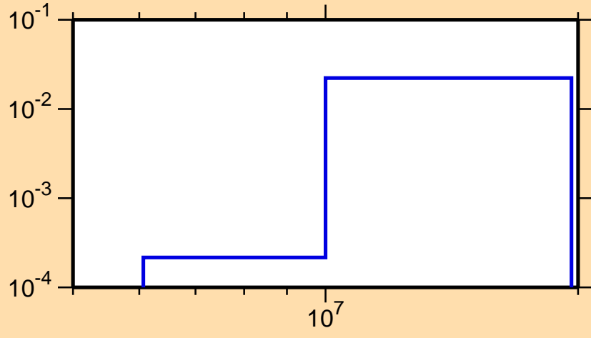
\sigma vs. E for ^{32}\text{S}(n,d)
