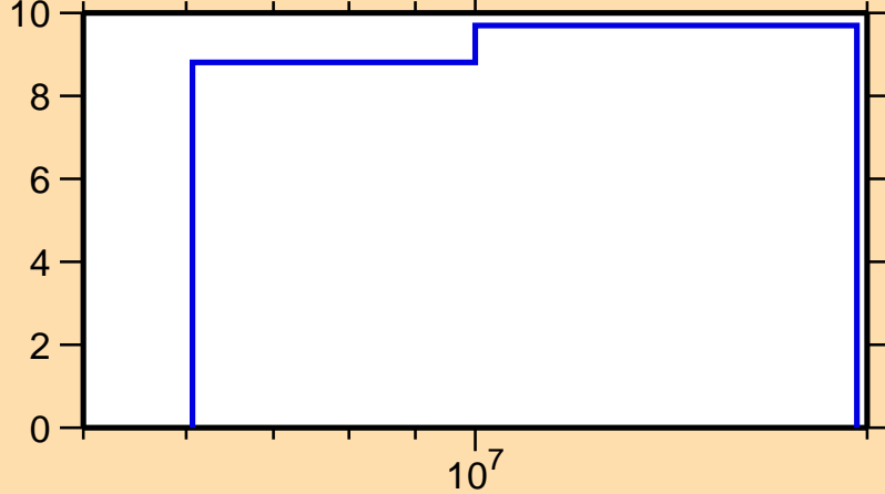
\Delta\sigma/\sigma vs. E for ^{32}\text{S}(n,ncont.)
