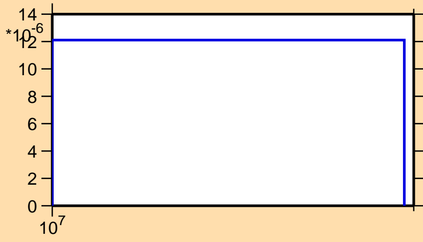
\sigma vs. E for ^{32}\text{S}(n,p\alpha)
