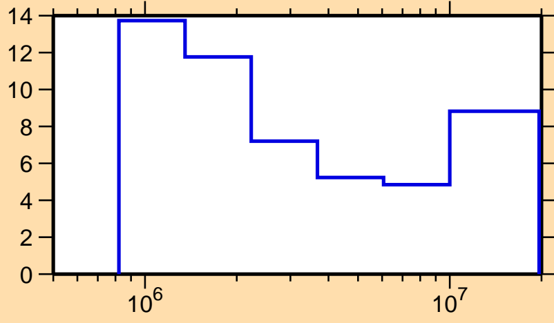
\Delta\sigma/\sigma vs. E for ^{32}\text{S}(n,p)
