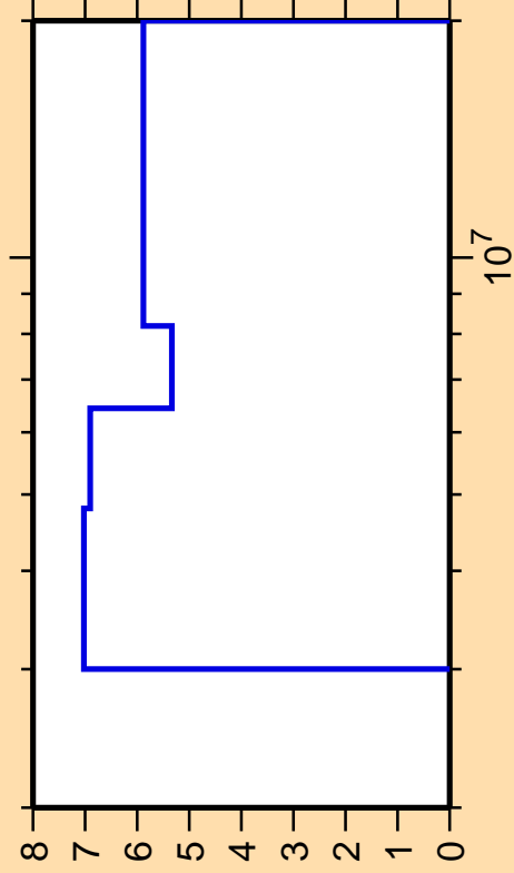
\Delta\sigma/\sigma vs. E for ^{32}\text{S}(n,n_4)
