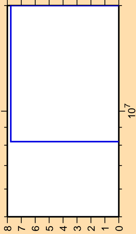
\Delta\sigma/\sigma vs. E for ^{32}\text{S}(n,p)
