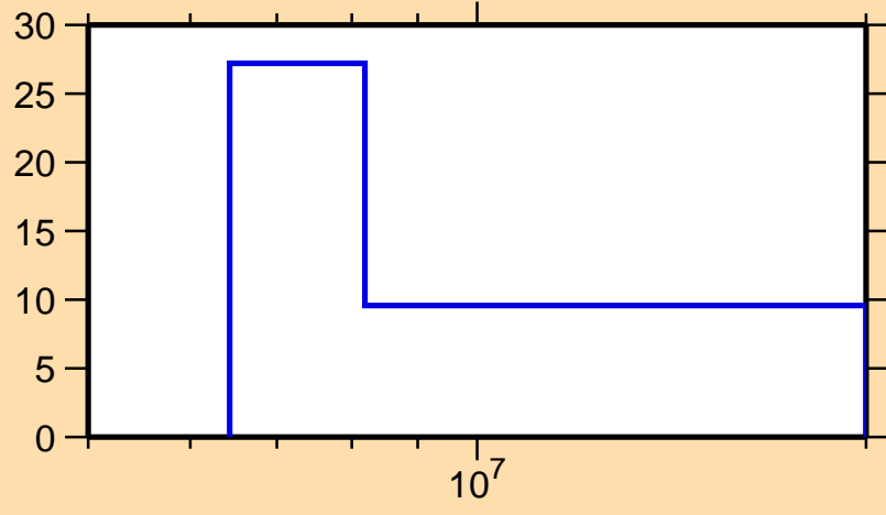
\Delta\sigma/\sigma vs. E for ^{32}\text{S}(n,n\text{cont.})
