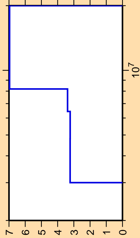
\Delta\sigma/\sigma vs. E for ^{32}\text{S}(n,n_2)
