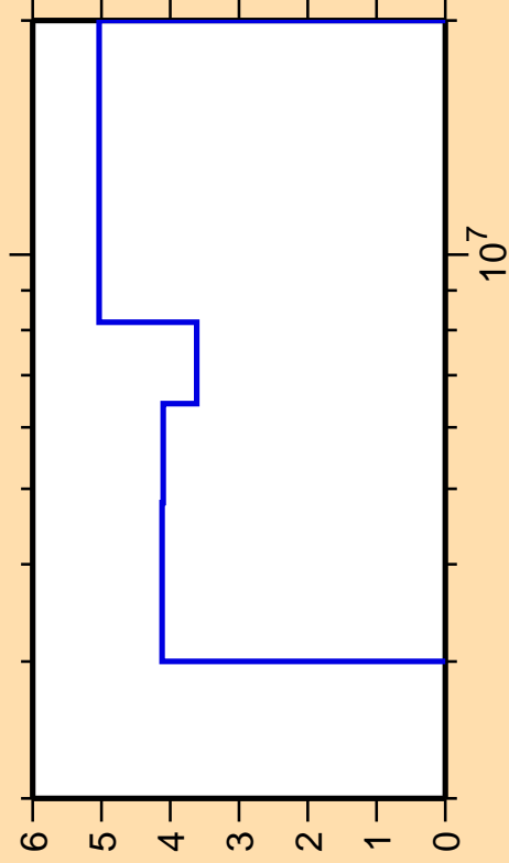
\Delta\sigma/\sigma vs. E for ^{32}\text{S}(n,n_3)
