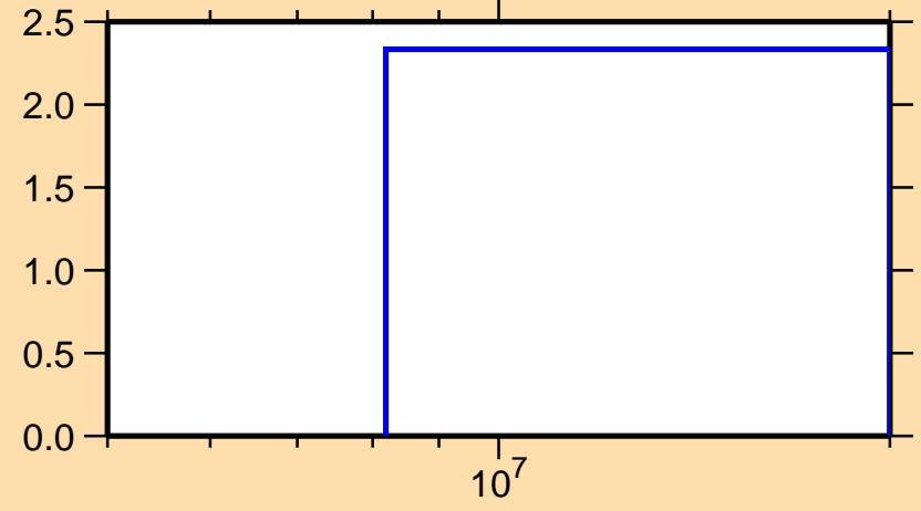
\Delta\sigma/\sigma vs. E for ^{32}\text{S}(n,\text{nonel.})
