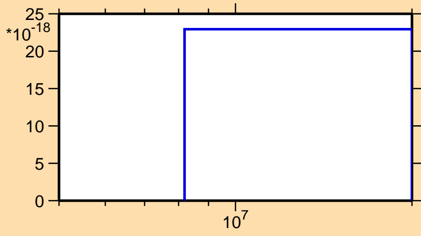
\sigma vs. E for ^{32}\text{S}(n,nd)
