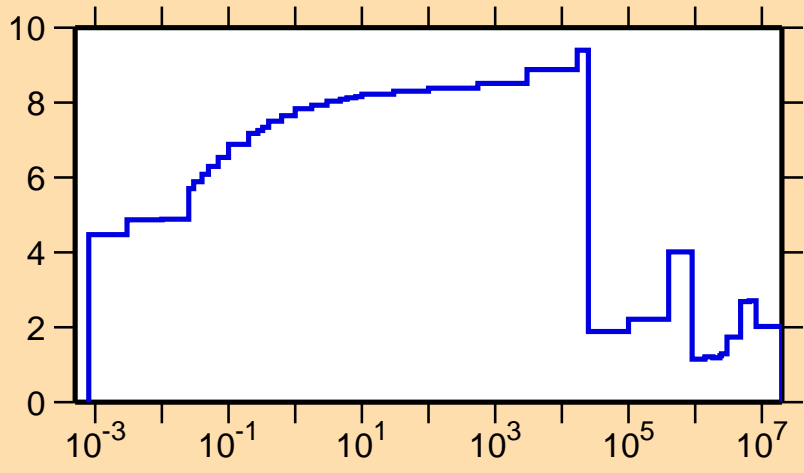
\Delta\sigma/\sigma vs. E for ^{32}\text{S}(n,\text{tot.})
