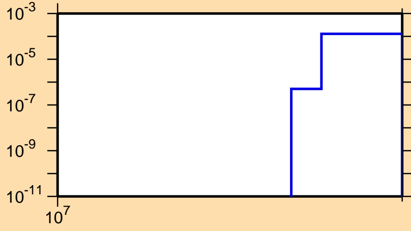
\sigma vs. E for ^{33}\text{S}(n,\text{nd})
