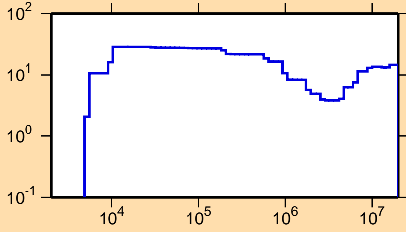
\Delta\sigma/\sigma vs. E for ^{33}\text{S}(n,p)
