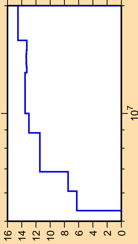
\Delta\sigma/\sigma vs. E for ^{33}\text{S}(n,p)
