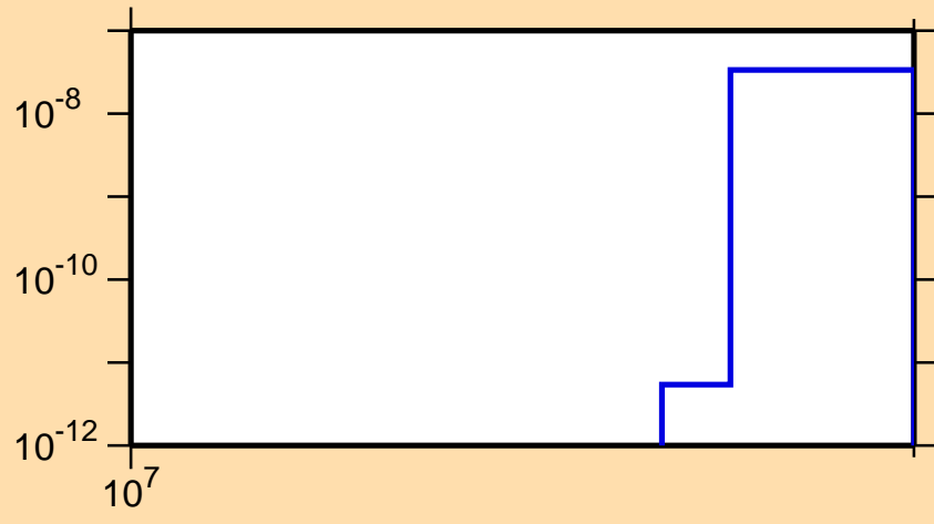
\sigma vs. E for ^{33}\text{S}(n,\text{pd})
