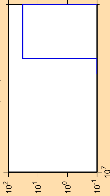
\Delta\sigma/\sigma vs. E for ^{33}\text{S}(n,\text{nd})
