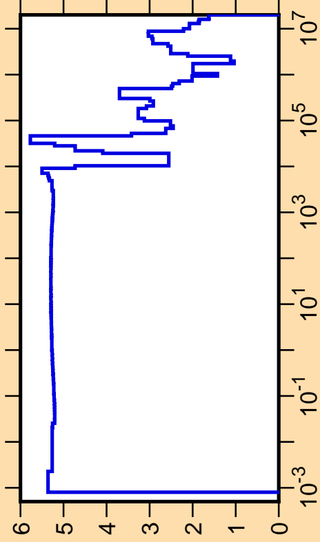
\Delta\sigma/\sigma vs. E for ^{33}\text{S}(n,\text{tot.})
