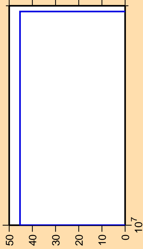
\Delta\sigma/\sigma vs. E for ^{33}\text{S}(n,pd)
