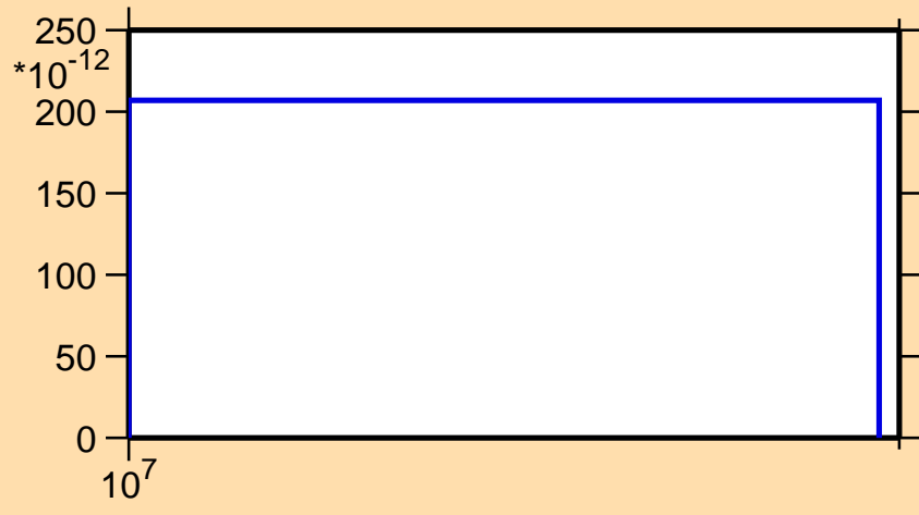
\sigma vs. E for ^{33}\text{S}(n,pd)
