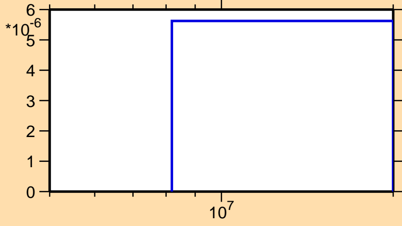
\sigma vs. E for ^{33}\text{S}(n,p\alpha)
