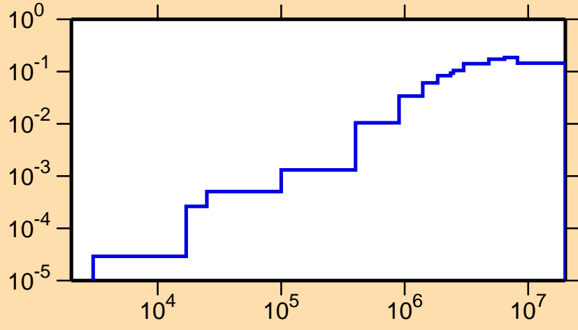
\sigma vs. E for ^{33}\text{S}(n,p)
