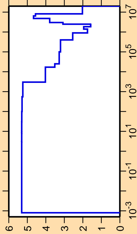
\Delta\sigma/\sigma vs. E for ^{33}\text{S}(n,\text{el.})
