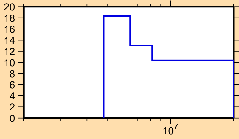
\Delta\sigma/\sigma vs. E for ^{33}\text{S}(n,n\text{cont.})
