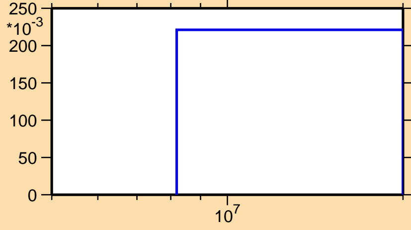
\sigma vs. E for ^{33}\text{S}(n,2n)
