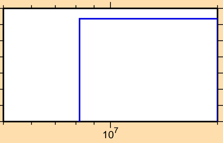
\sigma vs. E for ^{33}\text{S}(n,2np)
