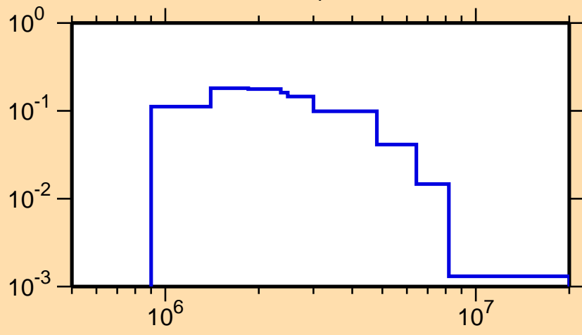
\sigma vs. E for ^{33}\text{S}(n,n_1)
