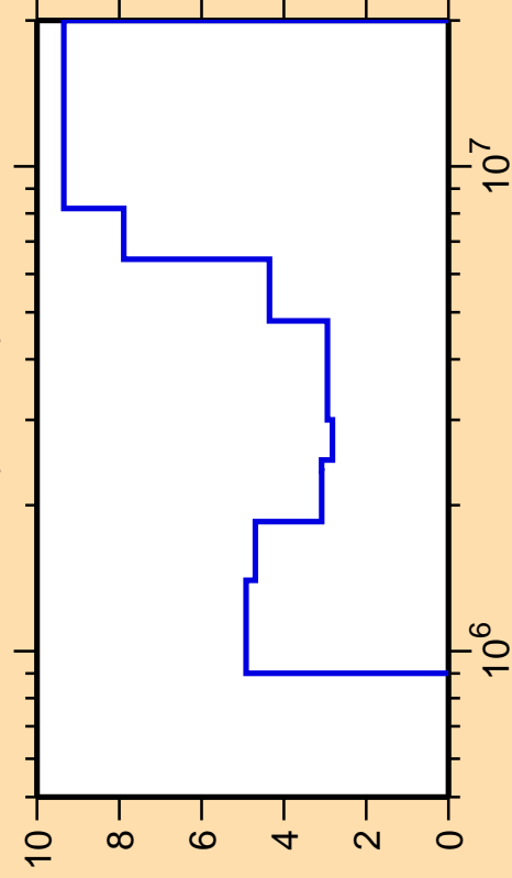
\Delta\sigma/\sigma vs. E for ^{33}\text{S}(n,\text{inel.})
