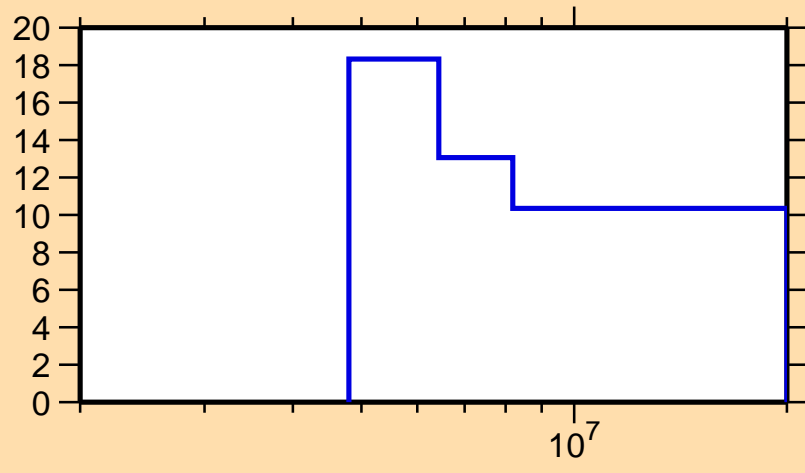
\Delta\sigma/\sigma vs. E for ^{33}\text{S}(n,ncont.)
