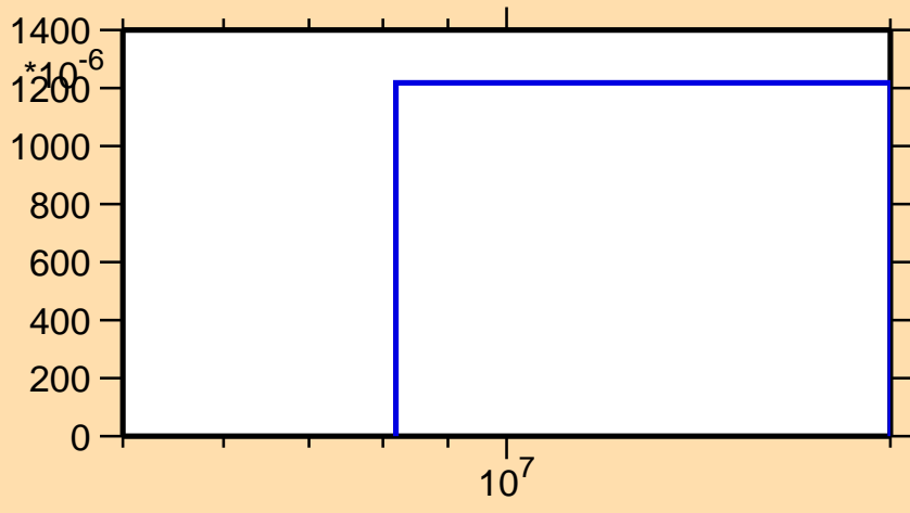
\sigma vs. E for ^{33}\text{S}(n,t)
