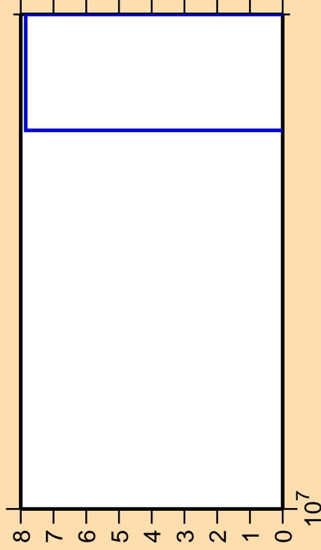
\Delta\sigma/\sigma vs. E for ^{34}\text{S}(n,2n\alpha)
