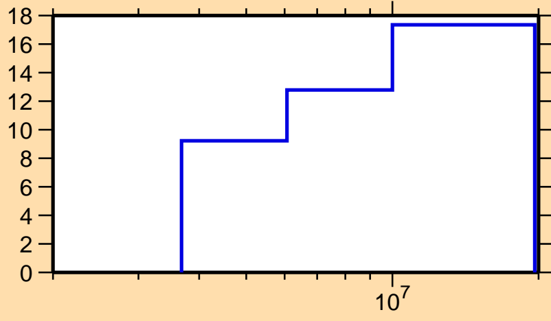
\Delta\sigma/\sigma vs. E for ^{34}\text{S}(n,p)
