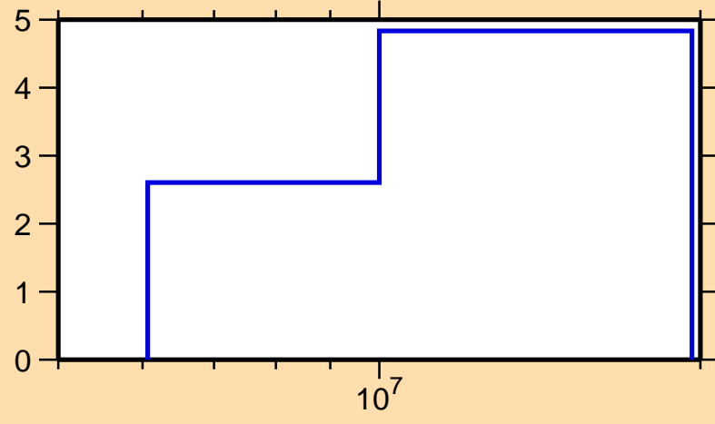
\Delta\sigma/\sigma vs. E for ^{34}\text{S}(n,\text{inel.})
