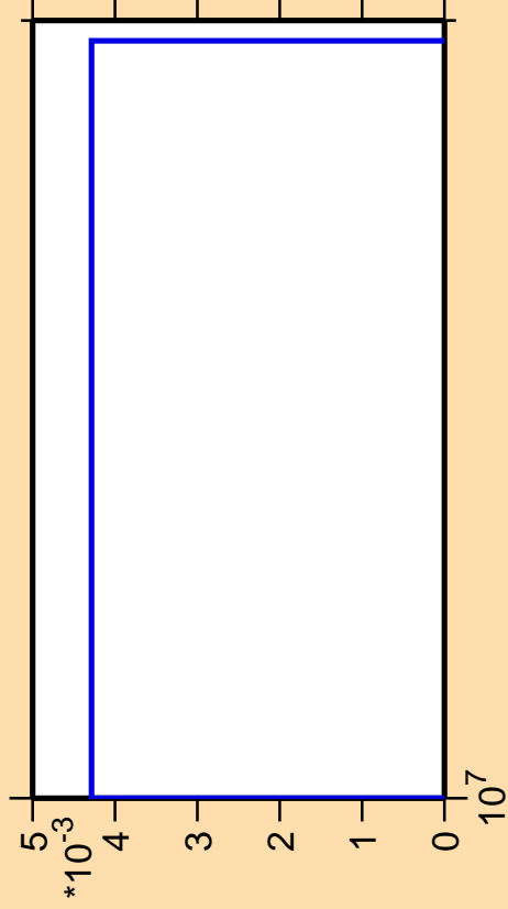
\Delta\sigma/\sigma vs. E for ^{34}\text{S}(n,pd)
