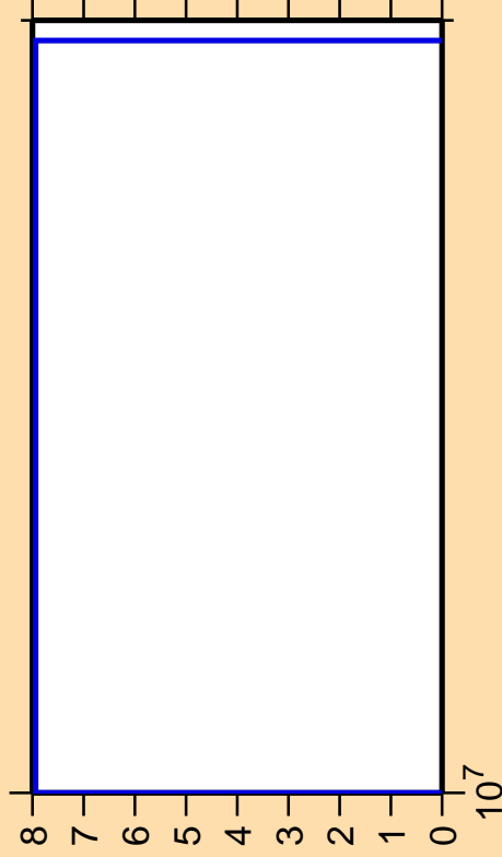
\Delta\sigma/\sigma vs. E for ^{34}\text{S}(n,\alpha)
