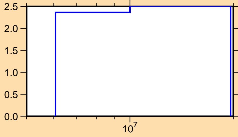
\Delta\sigma/\sigma vs. E for ^{34}\text{S}(n,n\text{onel.})
