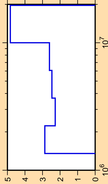
\Delta\sigma/\sigma vs. E for ^{34}\text{S}(n,\text{inel.})
