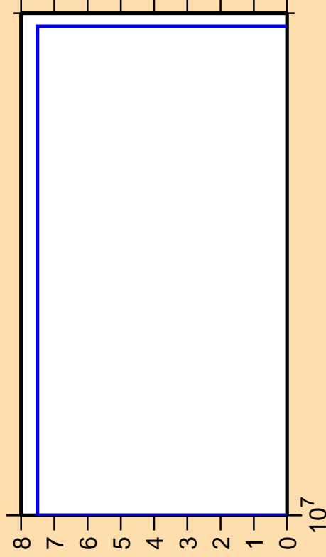
\Delta\sigma/\sigma vs. E for ^{34}\text{S}(n,n\text{cont.})
