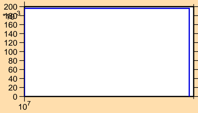
\sigma vs. E for ^{34}\text{S}(n,2n)
