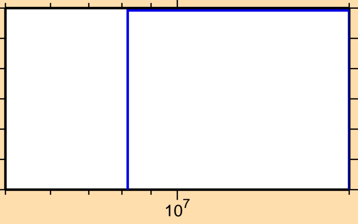
\sigma vs. E for ^{34}\text{S}(n,pd)
