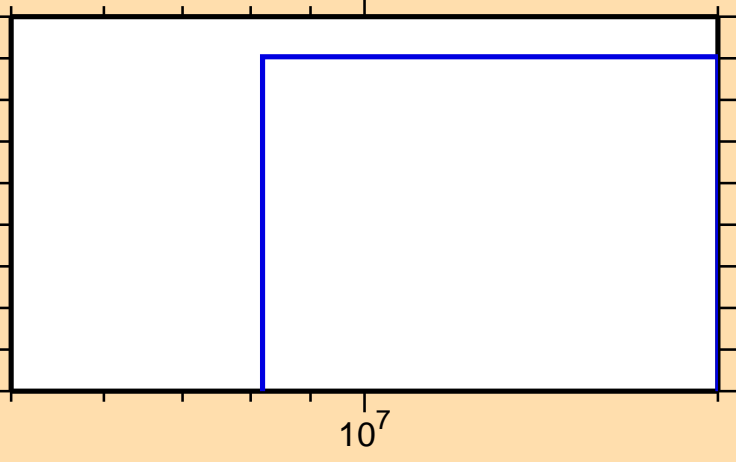
\sigma vs. E for ^{34}\text{S}(n,p\alpha)
