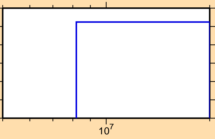
\sigma vs. E for ^{34}\text{S}(n,d)
