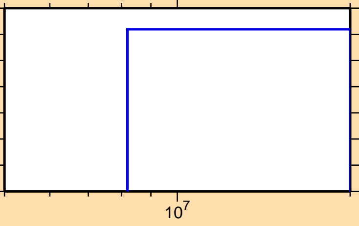
\sigma vs. E for ^{34}\text{S}(\text{mt117})
