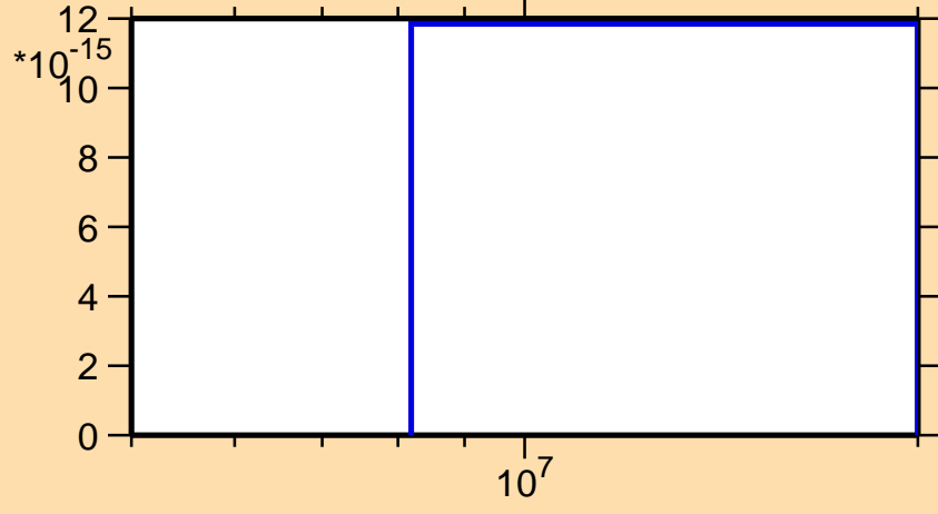
\sigma vs. E for ^{34}\text{S}(n,pd)
