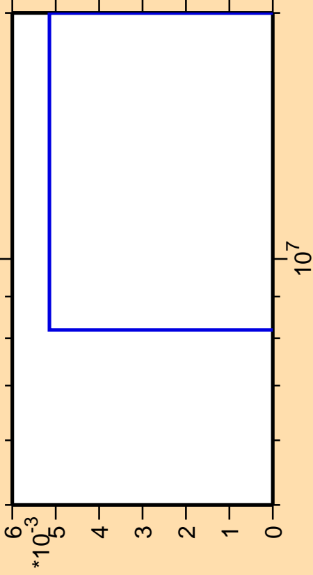
\Delta\sigma/\sigma vs. E for ^{34}\text{S}(n,pd)
