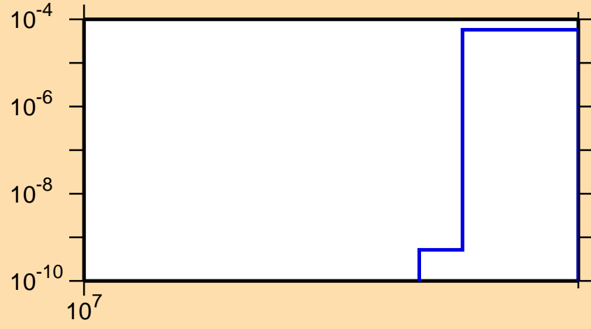
\sigma vs. E for ^{35}\text{S}(n,2n\alpha)
