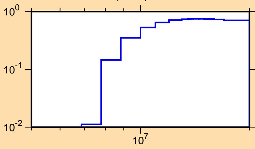
\sigma vs. E for ^{35}\text{S}(n,2n)
