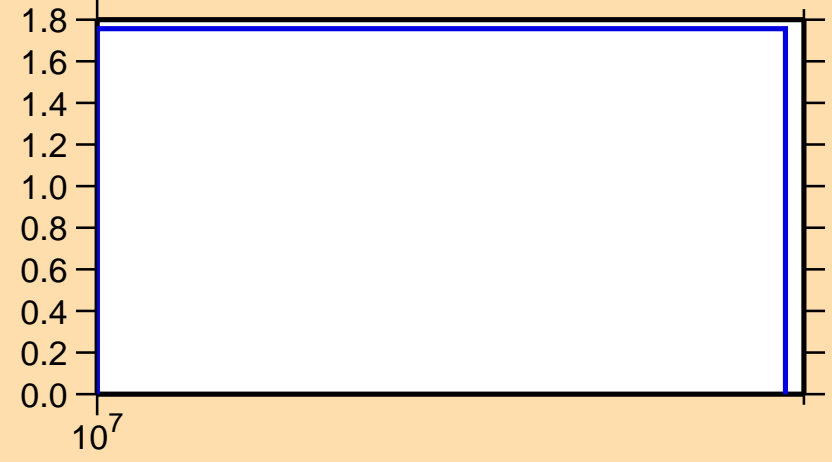
\Delta\sigma/\sigma vs. E for ^{36}\text{S}(n,\text{tot.})
