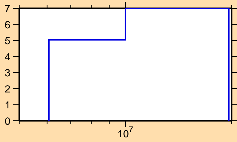
\Delta\sigma/\sigma vs. E for ^{36}\text{S}(n,ncont.)
