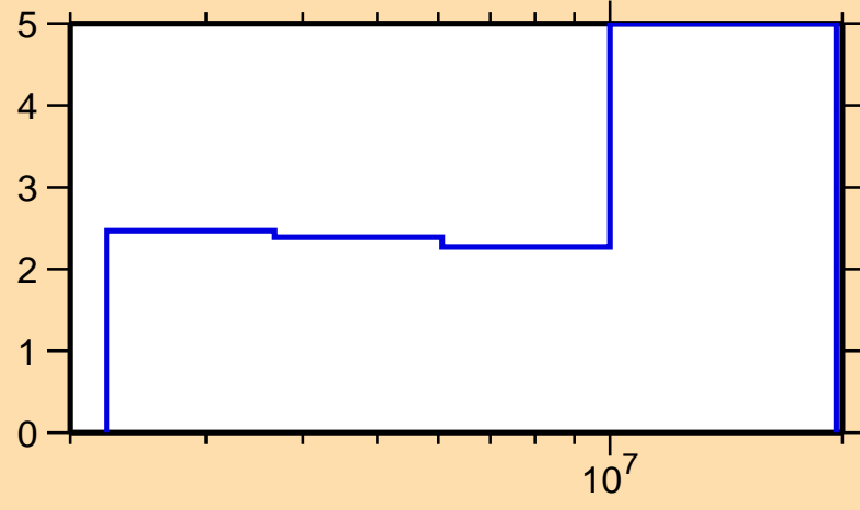
\Delta\sigma/\sigma vs. E for ^{36}\text{S}(n,\text{inel.})
