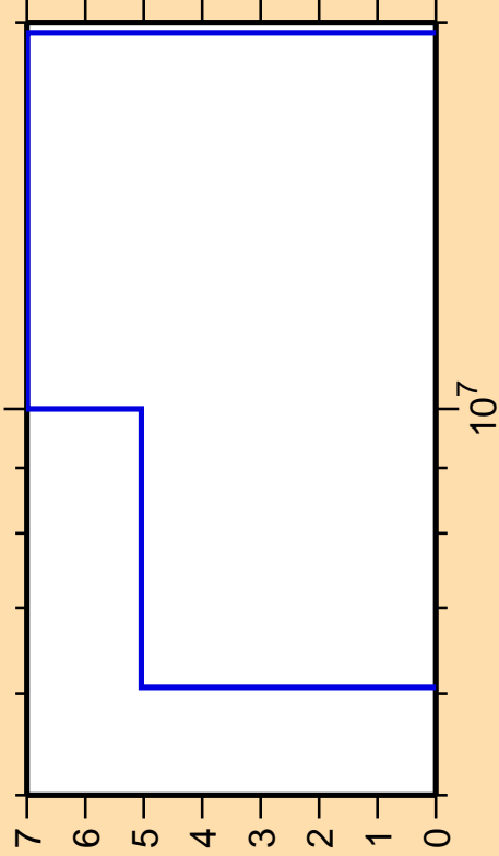
\Delta\sigma/\sigma vs. E for ^{36}\text{S}(n,n\text{cont.})
