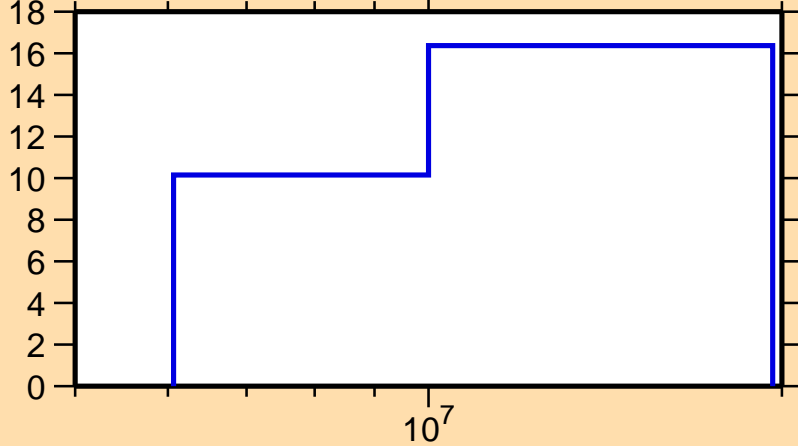
\Delta\sigma/\sigma vs. E for ^{37}\text{S}(n,ncont.)
