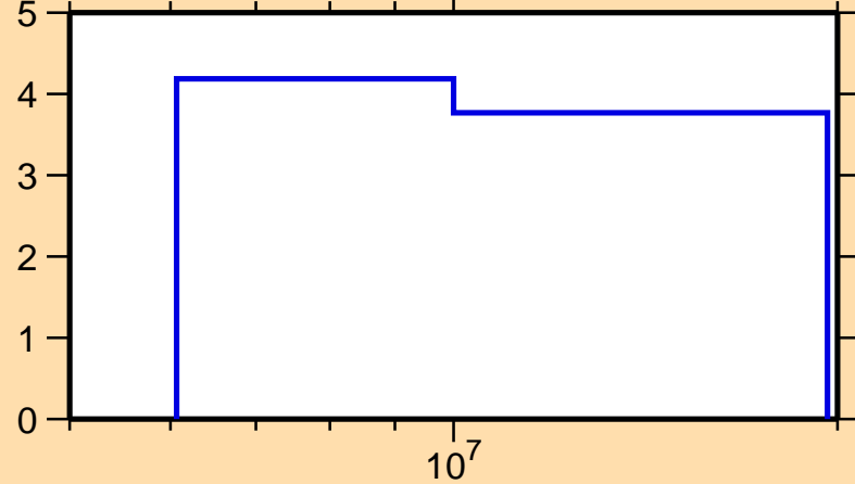
\Delta\sigma/\sigma vs. E for ^{37}\text{S}(n,2n)
