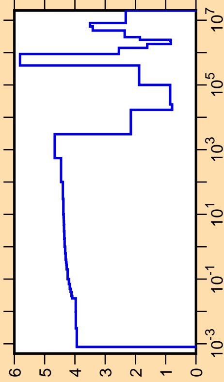
\Delta\sigma/\sigma vs. E for ^{37}\text{S}(n,\text{tot.})
