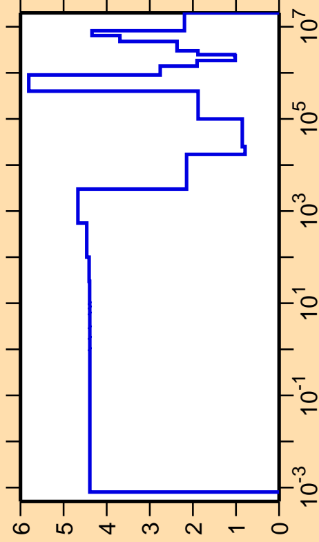
\Delta\sigma/\sigma vs. E for ^{37}\text{S}(n,\text{el.})
