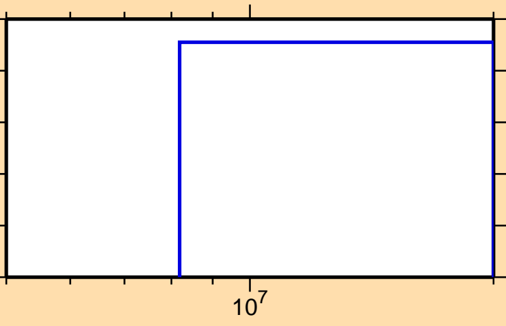
\sigma vs. E for ^{37}\text{S}(n,np)
