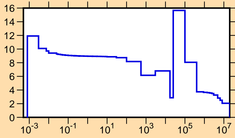
\sigma vs. E for ^{37}\text{S}(n,\text{tot.})
