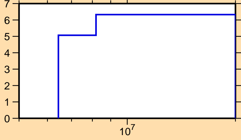
\Delta\sigma/\sigma vs. E for ^{37}\text{S}(n,\text{inel.})
