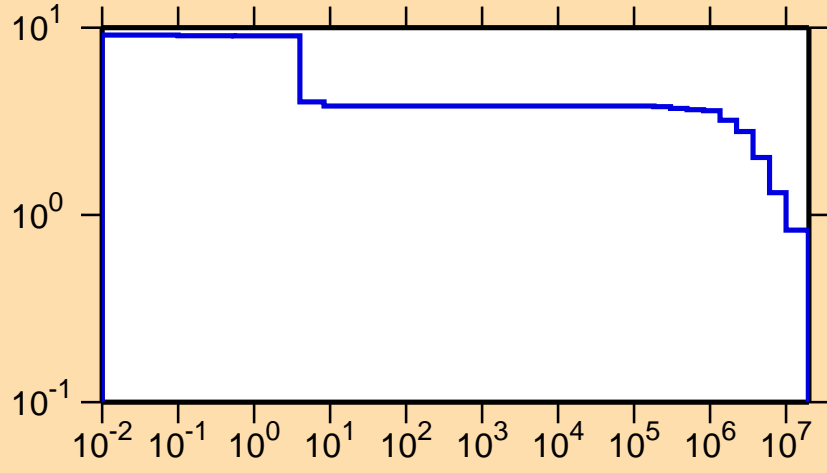
\sigma vs. E for ^{38}\text{S}(n,\text{el.})
