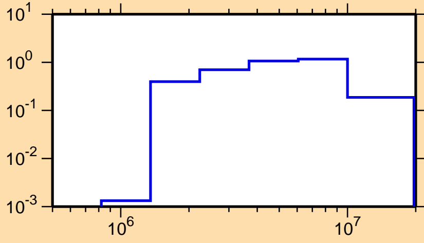
\sigma vs. E for ^{38}\text{S}(n,\text{inel.})
