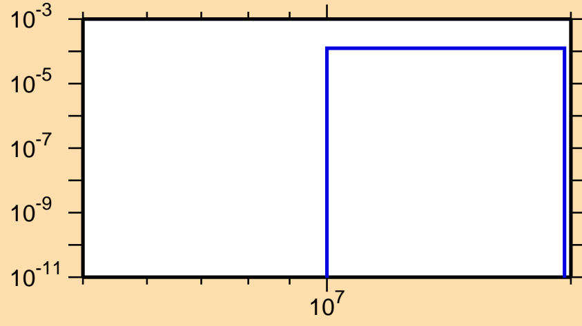
\sigma vs. E for ^{38}\text{S}(n,n\alpha)
