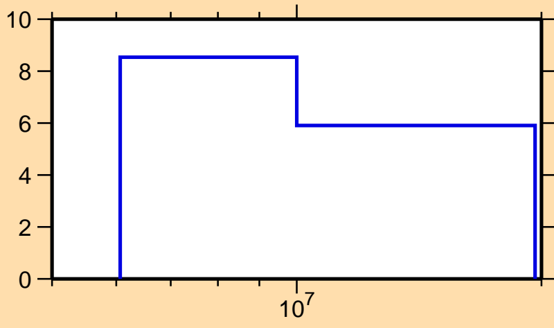
\Delta\sigma/\sigma vs. E for ^{38}\text{S}(n,\text{inel.})
