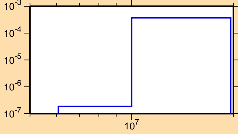
\sigma vs. E for ^{38}\text{S}(n,\alpha)
