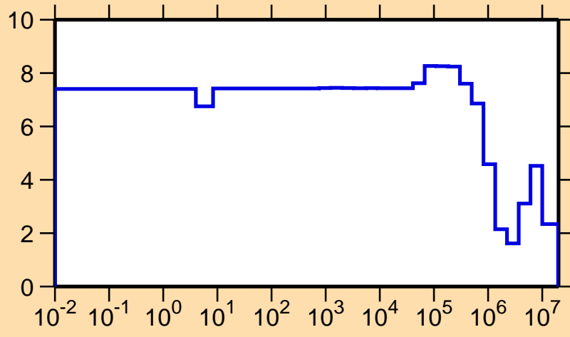
\Delta\sigma/\sigma vs. E for ^{38}\text{S}(n,\text{el.})
