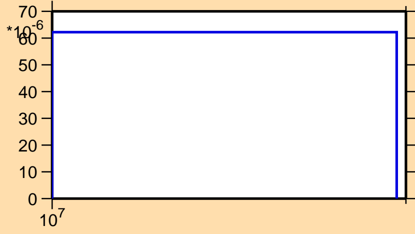
\sigma vs. E for ^{38}\text{S}(n,d)
