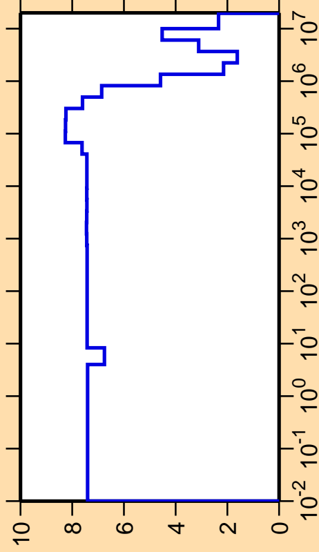
\Delta\sigma/\sigma vs. E for ^{38}\text{S}(n,\text{el.})
