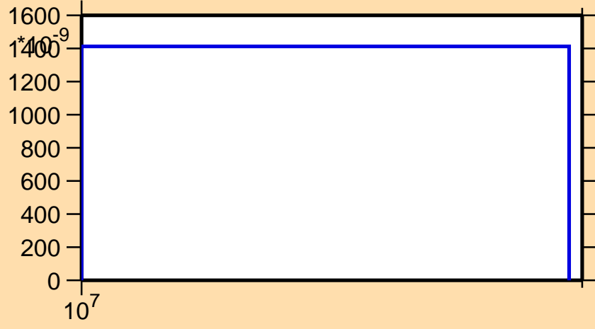
\sigma vs. E for ^{38}\text{S}(n,np)
