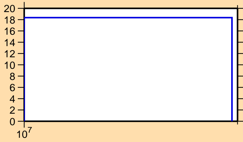
\Delta\sigma/\sigma vs. E for ^{38}\text{S}(n,ncont.)
