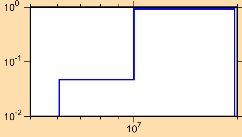
\sigma vs. E for ^{38}\text{S}(n,2n)
