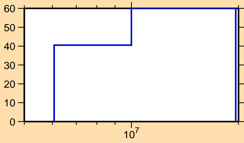
\Delta\sigma/\sigma vs. E for ^{38}\text{S}(n,\gamma)
