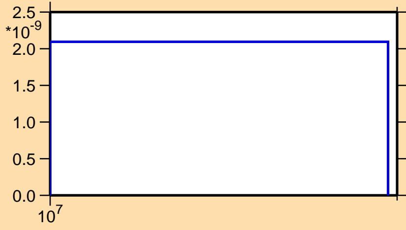
\sigma vs. E for ^{38}\text{S}(n,nt)
