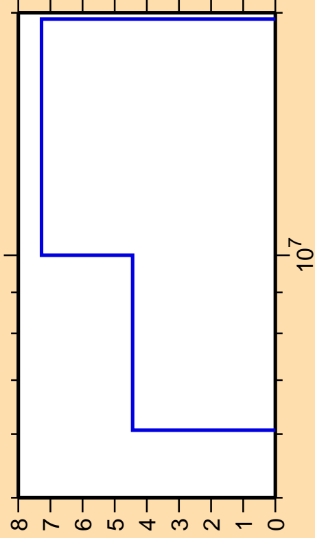
\Delta\sigma/\sigma vs. E for ^{38}\text{S}(n,2n)
