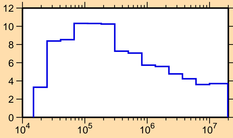
\Delta\sigma/\sigma vs. E for ^{38}\text{S}(n,\text{nonel.})
