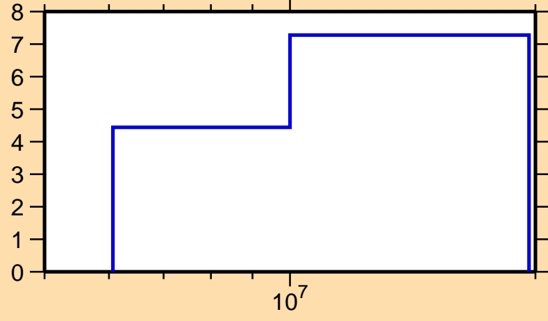
\Delta\sigma/\sigma vs. E for ^{38}\text{S}(n,2n)
