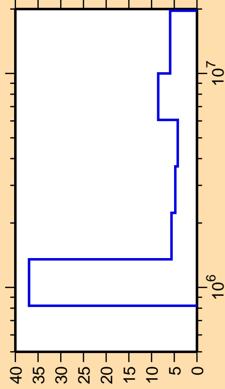
\Delta\sigma/\sigma vs. E for ^{38}\text{S}(n,\text{inel.})
