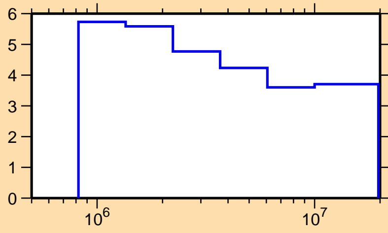
\Delta\sigma/\sigma vs. E for ^{38}\text{S}(n,\text{nonel.})
