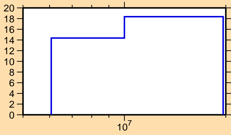
\Delta\sigma/\sigma vs. E for ^{38}\text{S}(n,n\text{cont.})
