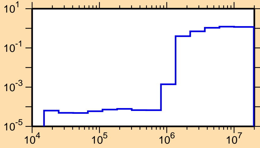
\sigma vs. E for ^{38}\text{S}(n,\text{nonel.})
