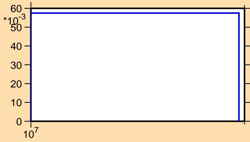
\sigma vs. E for ^{38}\text{S}(n,3n)
