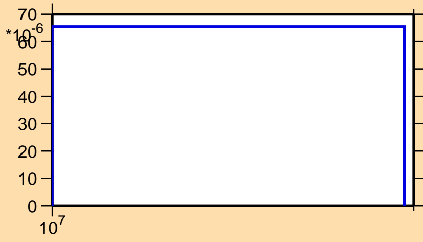
\sigma vs. E for ^{38}\text{S}(n,p)
