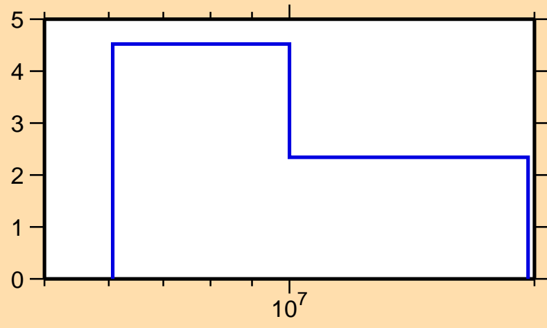
\Delta\sigma/\sigma vs. E for ^{38}\text{S}(n,\text{el.})
