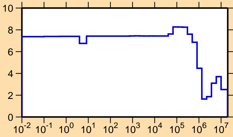
\Delta\sigma/\sigma vs. E for ^{38}\text{S}(n,\text{tot.})
